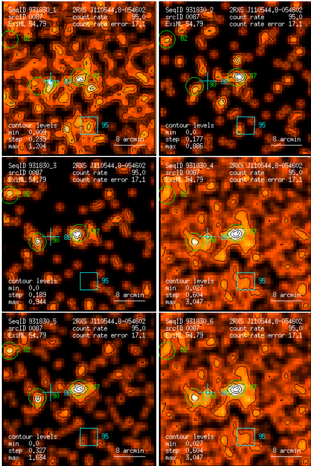
Figure 87: RASS 931830: detection 0087: band rate images, Gaussian filter: (1) PSPC channels 11 – 41, (2) 52 – 90, (3) 91 – 201, (4) 11 – 235, (5) 52 – 201, (6) 11 – 201. Broad band rates in counts/ks. Band rate contour levels in counts/ks/arcmin 2 .
