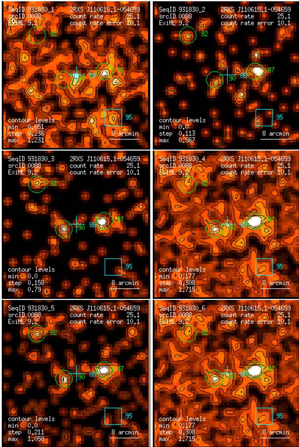
Figure 88: RASS 931830: detection 0088: band rate images, Gaussian filter: (1) PSPC channels 11 – 41, (2) 52 – 90, (3) 91 – 201, (4) 11 – 235, (5) 52 – 201, (6) 11 – 201. Broad band rates in counts/ks. Band rate contour levels in counts/ks/arcmin 2 .
