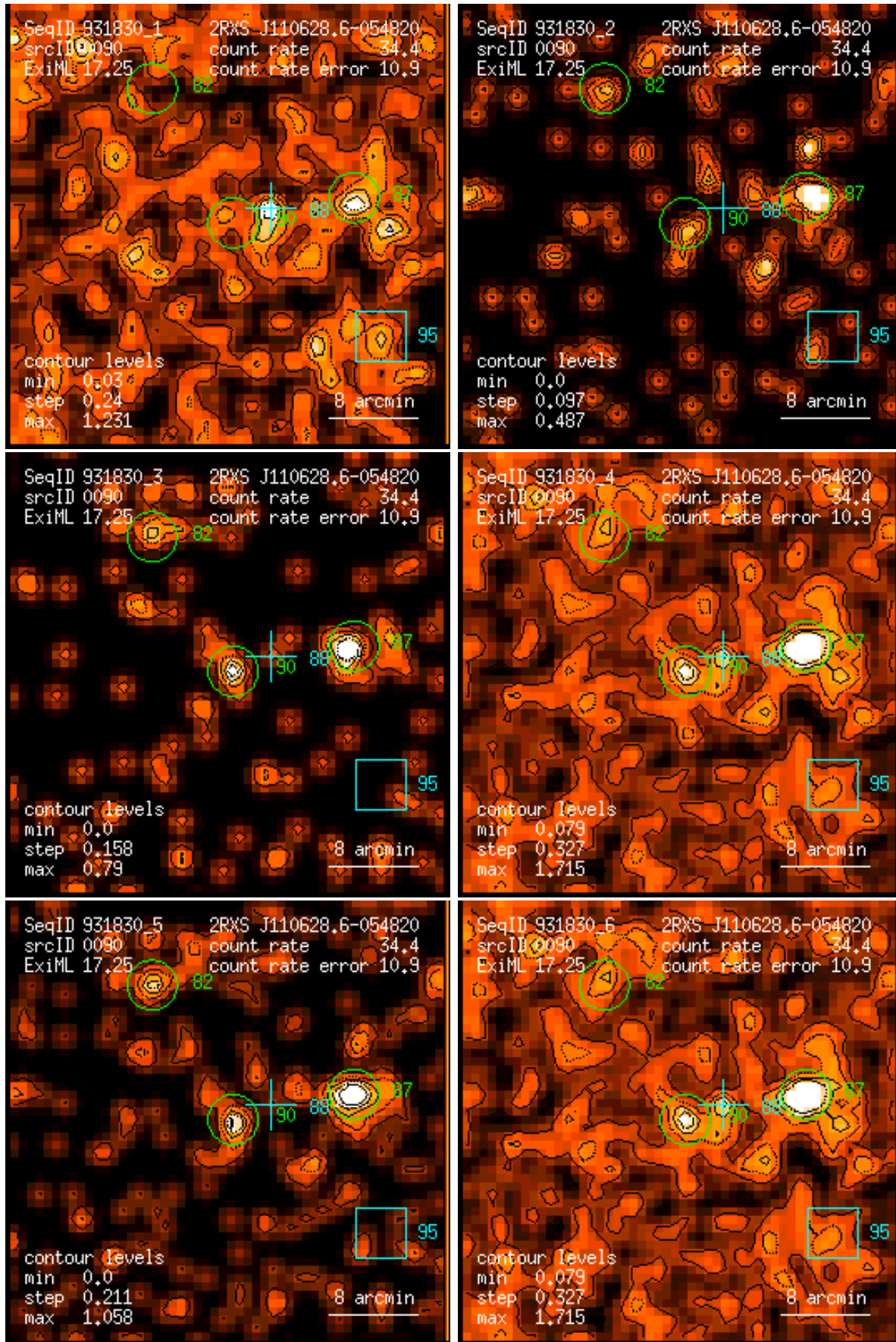
Figure 90: RASS 931830: detection 0090: band rate images, Gaussian filter: (1) PSPC channels 11 – 41, (2) 52 – 90, (3) 91 – 201, (4) 11 – 235, (5) 52 – 201, (6) 11 – 201. Broad band rates in counts/ks. Band rate contour levels in counts/ks/arcmin 2 .
