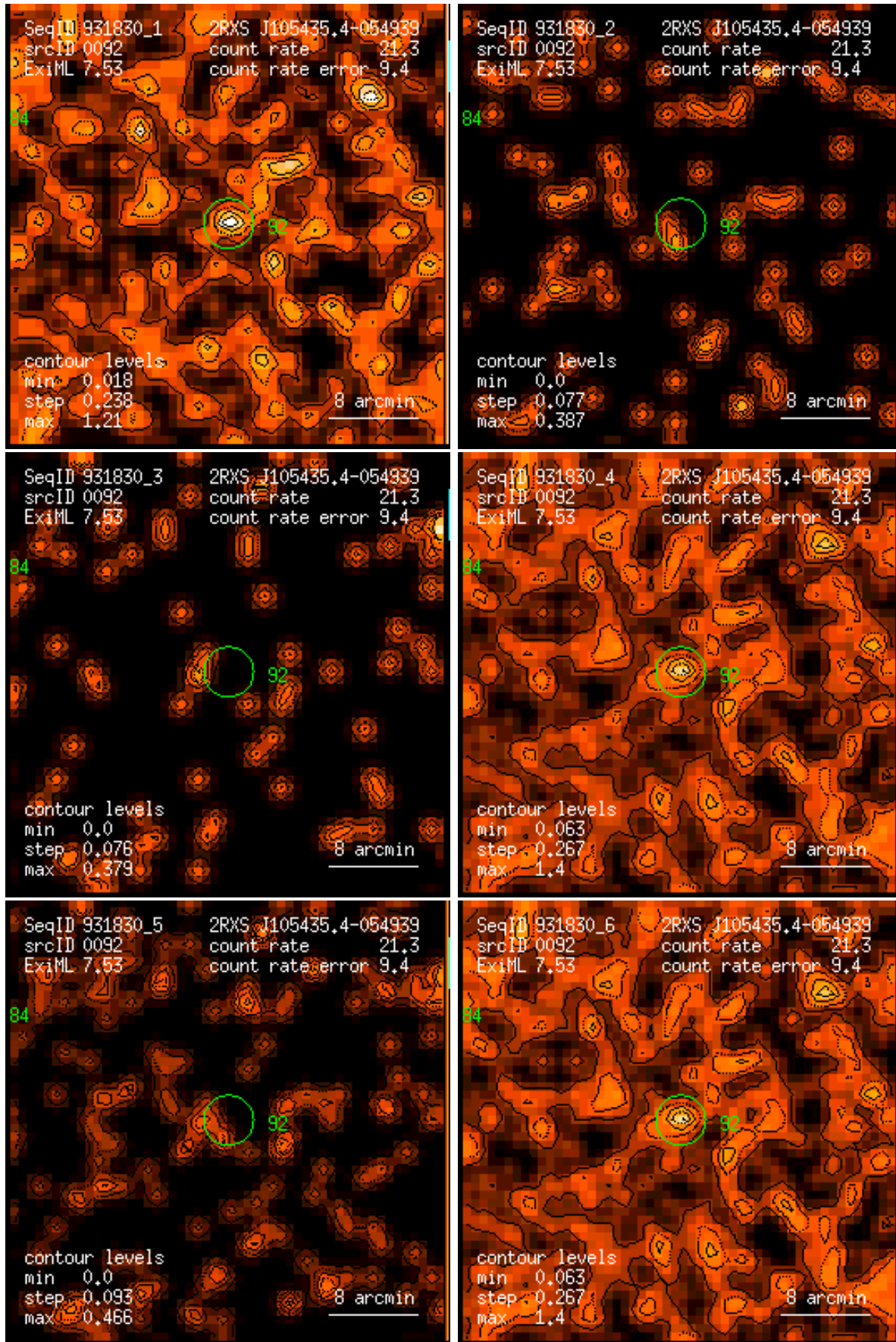
Figure 92: RASS 931830: detection 0092: band rate images, Gaussian filter: (1) PSPC channels 11 – 41, (2) 52 – 90, (3) 91 – 201, (4) 11 – 235, (5) 52 – 201, (6) 11 – 201. Broad band rates in counts/ks. Band rate contour levels in counts/ks/arcmin 2 .
