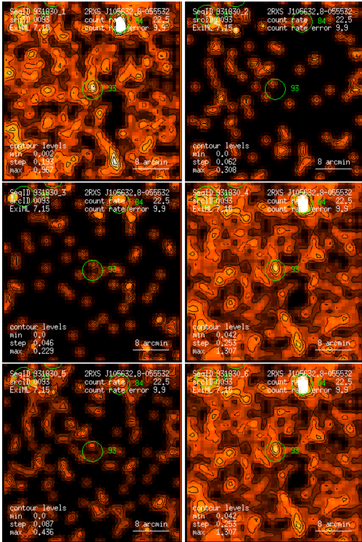
Figure 93: RASS 931830: detection 0093: band rate images, Gaussian filter: (1) PSPC channels 11 – 41, (2) 52 – 90, (3) 91 – 201, (4) 11 – 235, (5) 52 – 201, (6) 11 – 201. Broad band rates in counts/ks. Band rate contour levels in counts/ks/arcmin 2 .
