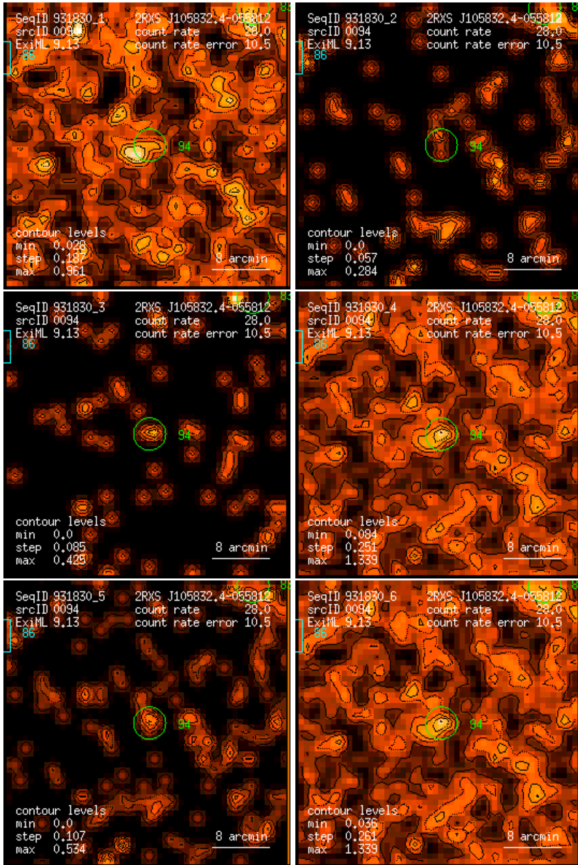
Figure 94: RASS 931830: detection 0094: band rate images, Gaussian filter: (1) PSPC channels 11 – 41, (2) 52 – 90, (3) 91 – 201, (4) 11 – 235, (5) 52 – 201, (6) 11 – 201. Broad band rates in counts/ks. Band rate contour levels in counts/ks/arcmin 2 .
