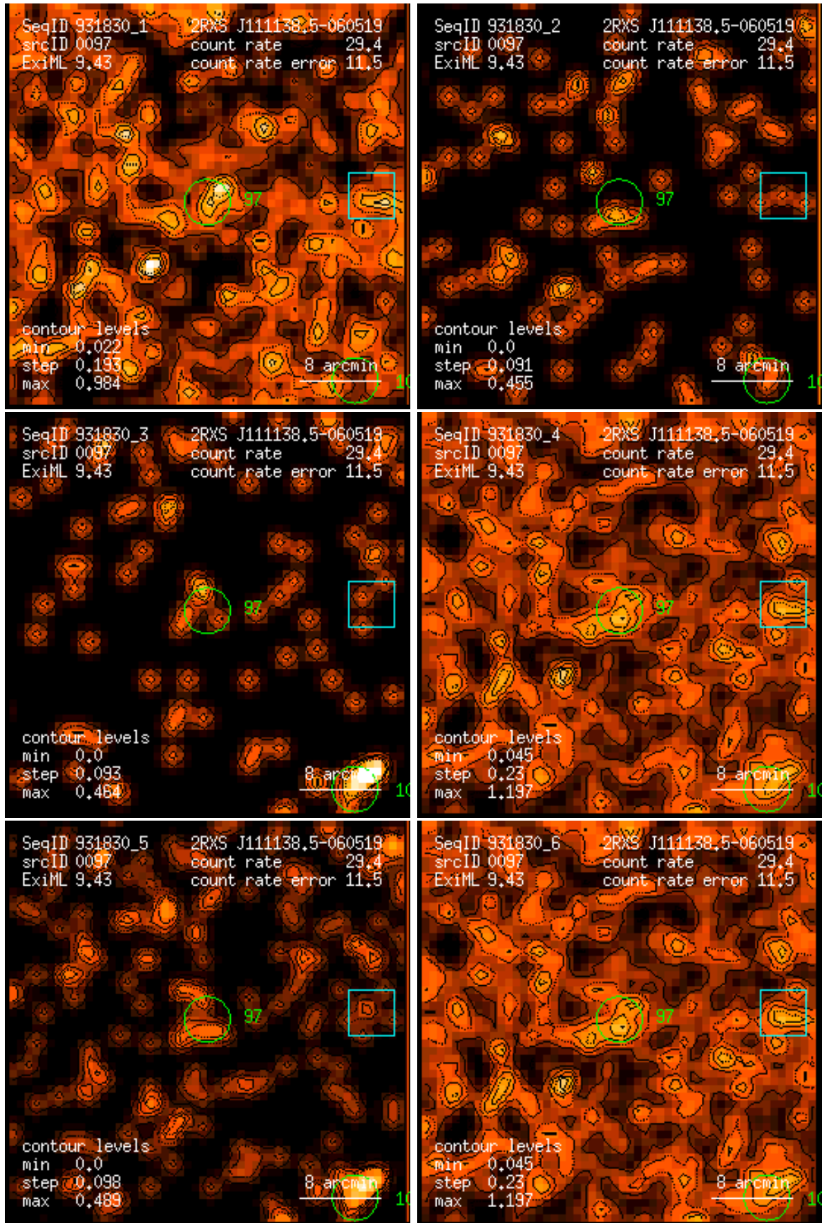
Figure 97: RASS 931830: detection 0097: band rate images, Gaussian filter: (1) PSPC channels 11 – 41, (2) 52 – 90, (3) 91 – 201, (4) 11 – 235, (5) 52 – 201, (6) 11 – 201. Broad band rates in counts/ks. Band rate contour levels in counts/ks/arcmin 2 .
