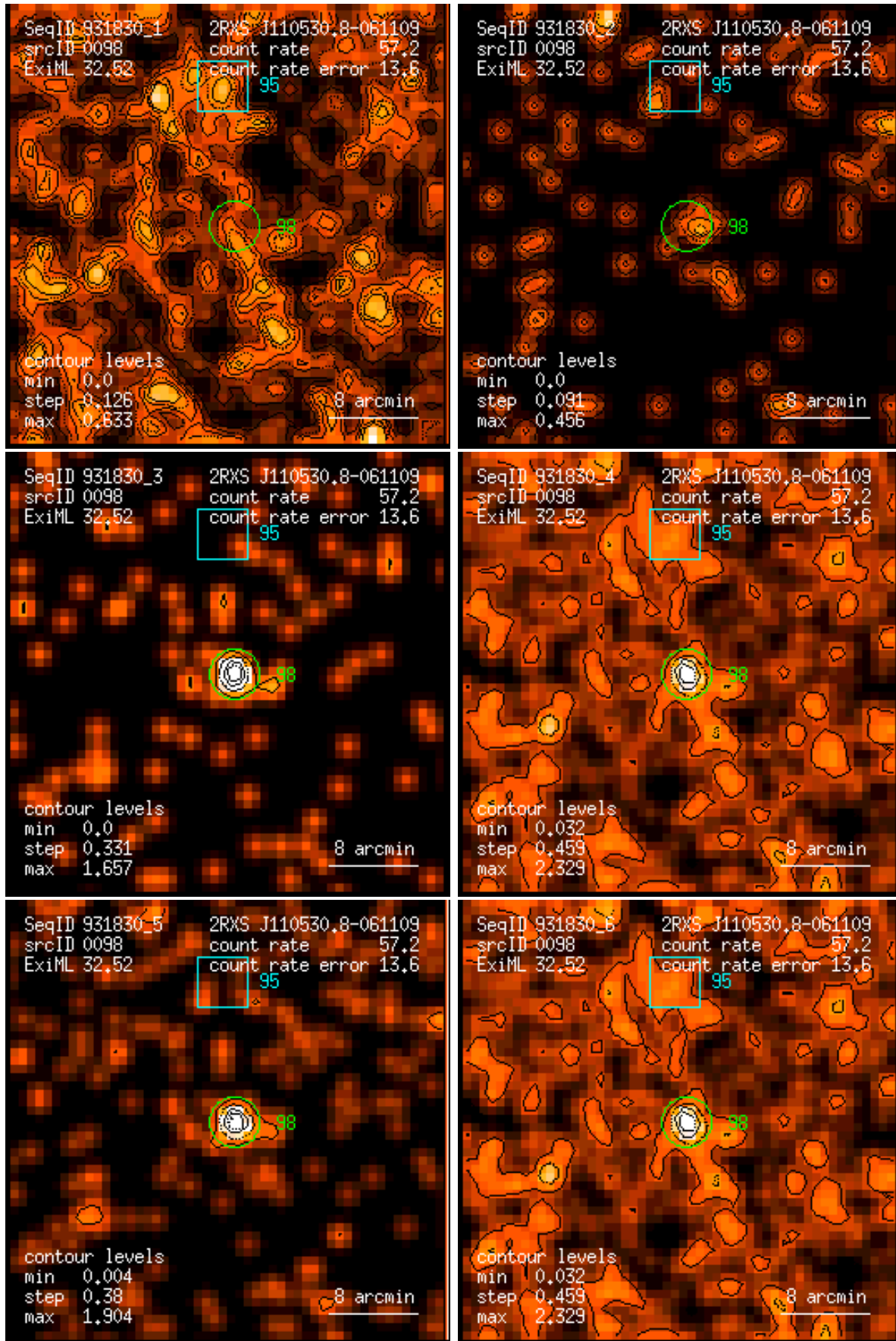
Figure 98: RASS 931830: detection 0098: band rate images, Gaussian filter: (1) PSPC channels 11 – 41, (2) 52 – 90, (3) 91 – 201, (4) 11 – 235, (5) 52 – 201, (6) 11 – 201. Broad band rates in counts/ks. Band rate contour levels in counts/ks/arcmin 2 .
