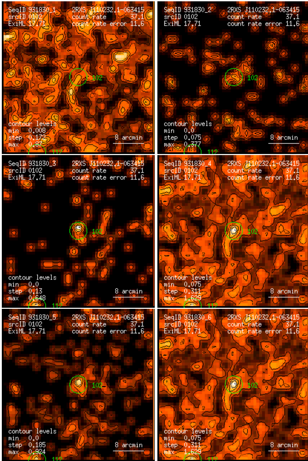
Figure 102: RASS 931830: detection 0102: band rate images, Gaussian filter: (1) PSPC channels 11 – 41, (2) 52 – 90, (3) 91 – 201, (4) 11 – 235, (5) 52 – 201, (6) 11 – 201. Broad band rates in counts/ks. Band rate contour levels in counts/ks/arcmin 2 .
