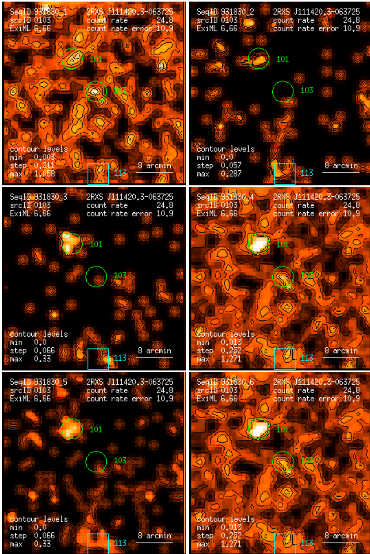
Figure 103: RASS 931830: detection 0103: band rate images, Gaussian filter: (1) PSPC channels 11 – 41, (2) 52 – 90, (3) 91 – 201, (4) 11 – 235, (5) 52 – 201, (6) 11 – 201. Broad band rates in counts/ks. Band rate contour levels in counts/ks/arcmin 2 .
