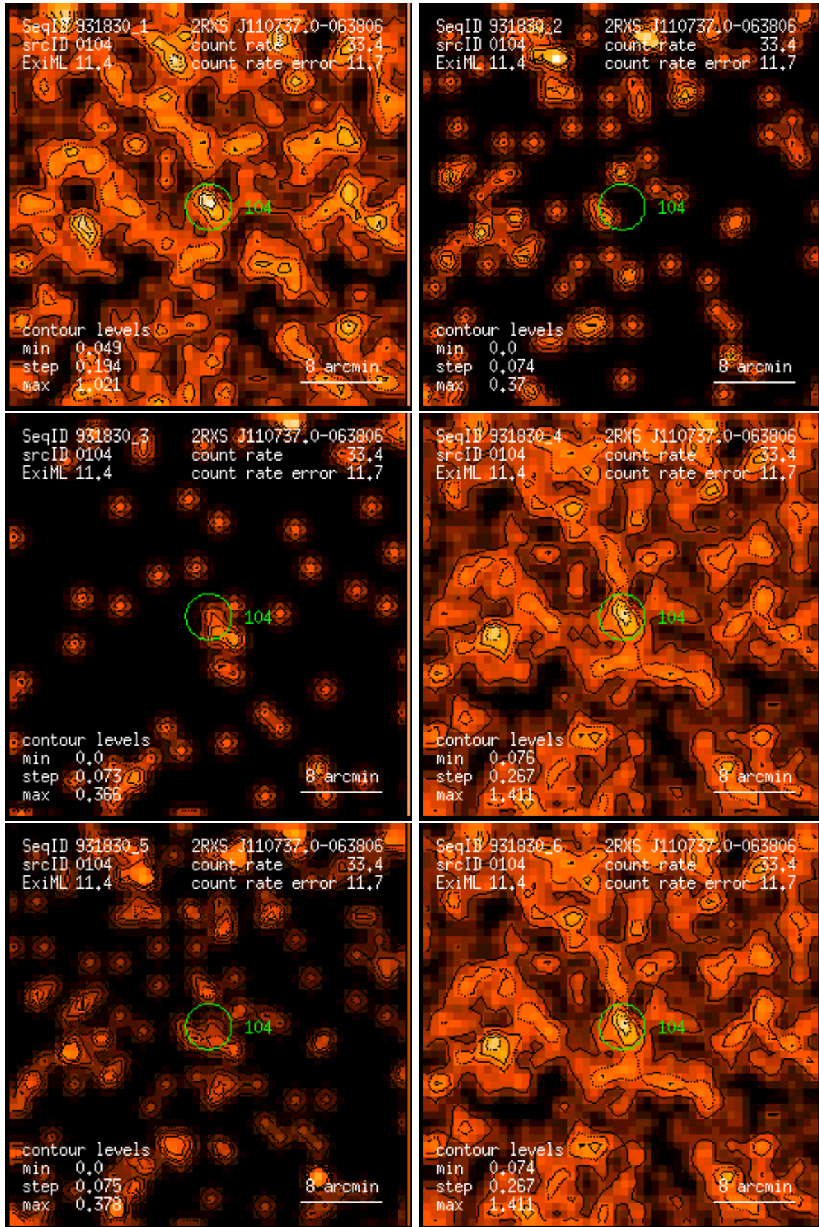
Figure 104: RASS 931830: detection 0104: band rate images, Gaussian filter: (1) PSPC channels 11 – 41, (2) 52 – 90, (3) 91 – 201, (4) 11 – 235, (5) 52 – 201, (6) 11 – 201. Broad band rates in counts/ks. Band rate contour levels in counts/ks/arcmin 2 .
