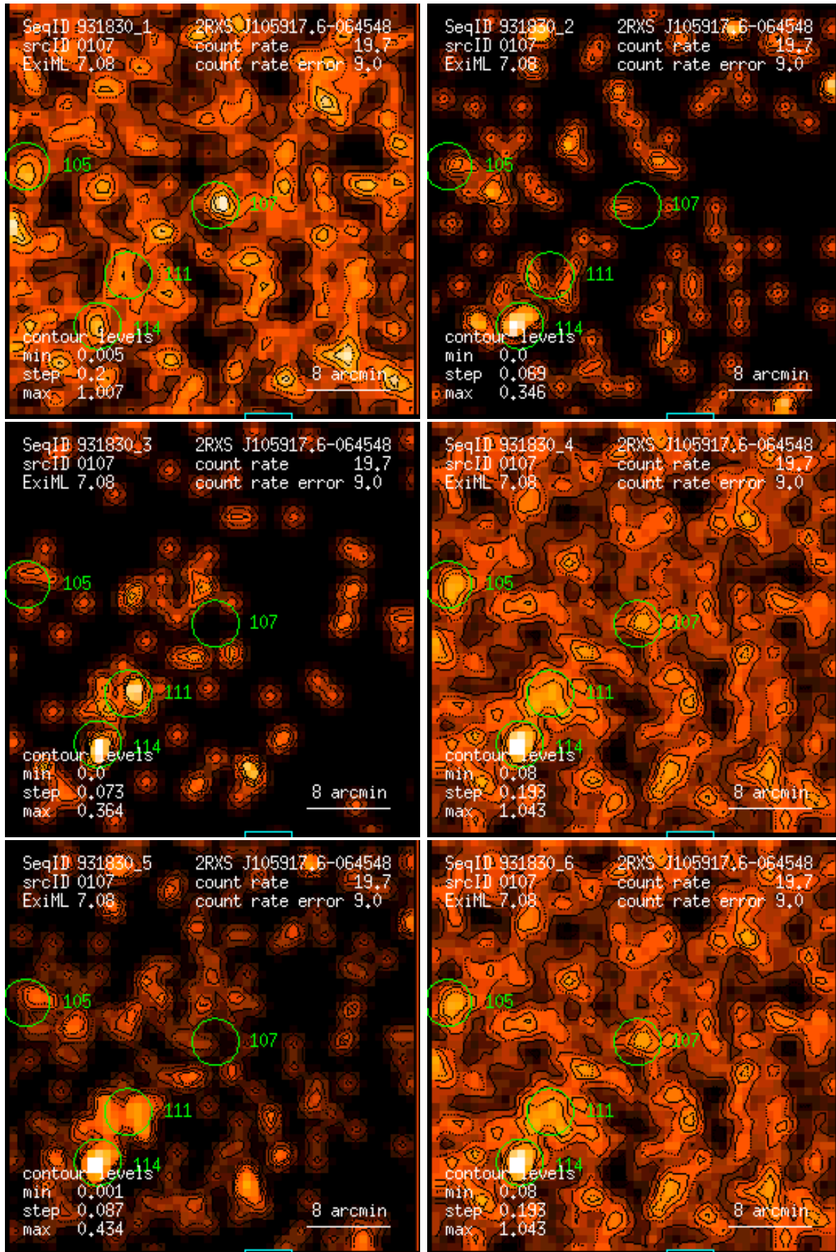
Figure 107: RASS 931830: detection 0107: band rate images, Gaussian filter: (1) PSPC channels 11 – 41, (2) 52 – 90, (3) 91 – 201, (4) 11 – 235, (5) 52 – 201, (6) 11 – 201. Broad band rates in counts/ks. Band rate contour levels in counts/ks/arcmin 2 .
