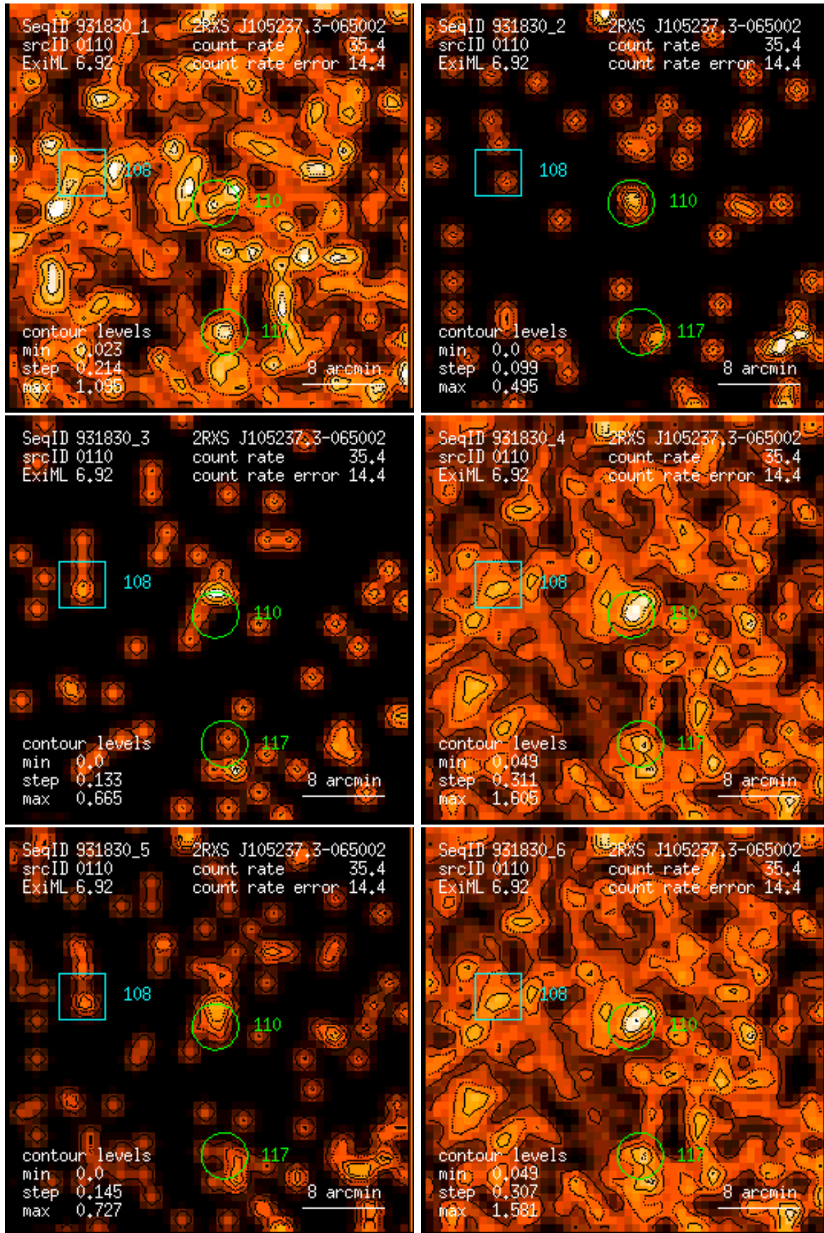
Figure 110: RASS 931830: detection 0110: band rate images, Gaussian filter: (1) PSPC channels 11 – 41, (2) 52 – 90, (3) 91 – 201, (4) 11 – 235, (5) 52 – 201, (6) 11 – 201. Broad band rates in counts/ks. Band rate contour levels in counts/ks/arcmin 2 .
