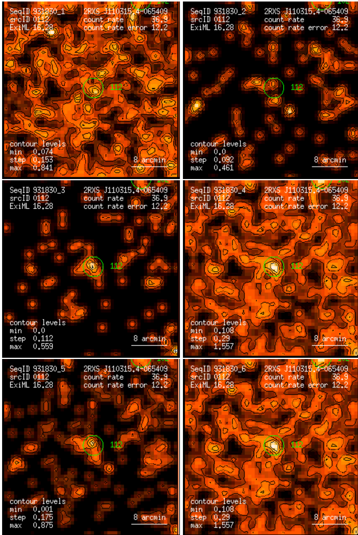
Figure 112: RASS 931830: detection 0112: band rate images, Gaussian filter: (1) PSPC channels 11 – 41, (2) 52 – 90, (3) 91 – 201, (4) 11 – 235, (5) 52 – 201, (6) 11 – 201. Broad band rates in counts/ks. Band rate contour levels in counts/ks/arcmin 2 .
