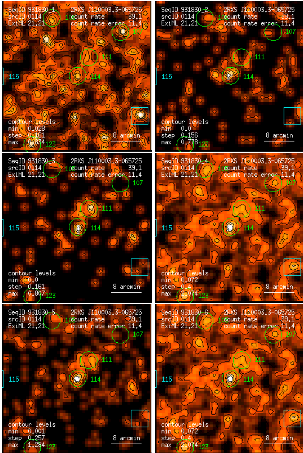
Figure 114: RASS 931830: detection 0114: band rate images, Gaussian filter: (1) PSPC channels 11 – 41, (2) 52 – 90, (3) 91 – 201, (4) 11 – 235, (5) 52 – 201, (6) 11 – 201. Broad band rates in counts/ks. Band rate contour levels in counts/ks/arcmin 2 .
