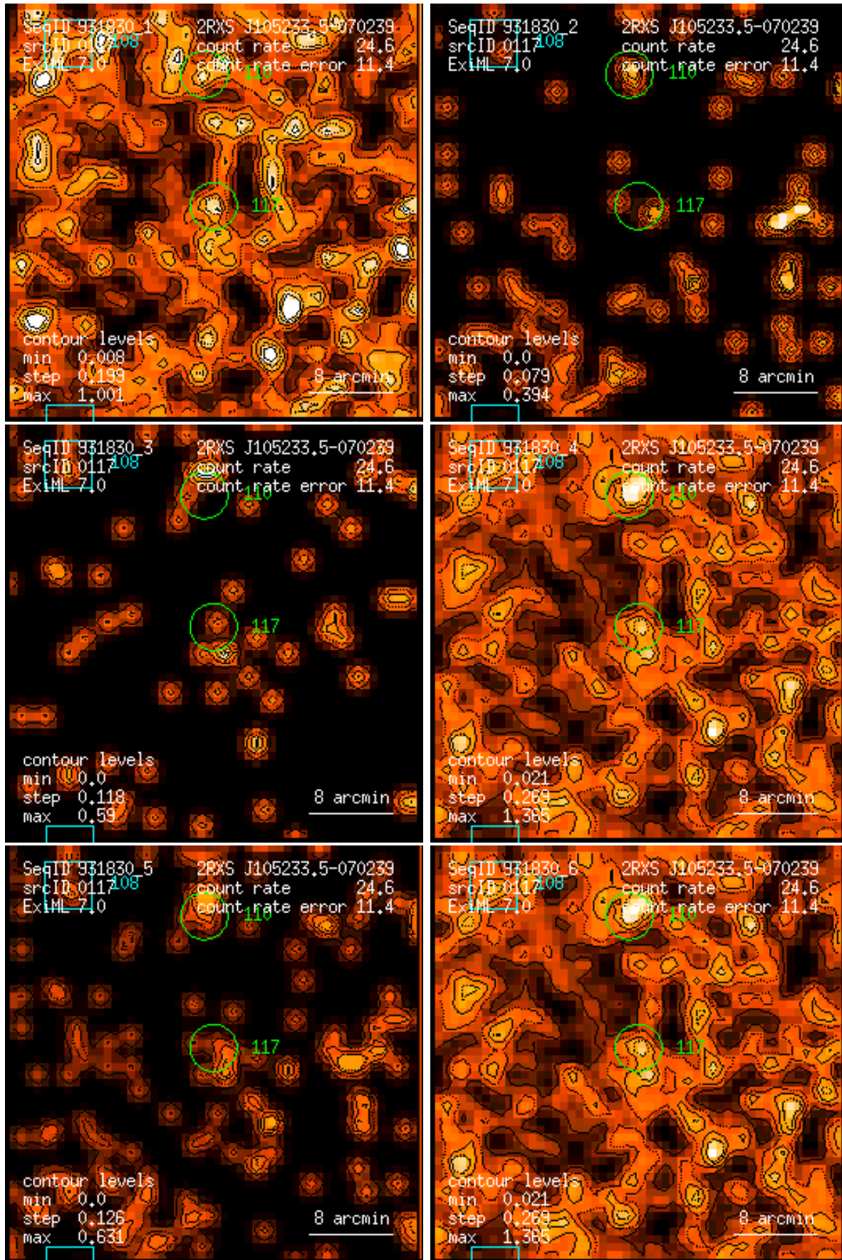
Figure 117: RASS 931830: detection 0117: band rate images, Gaussian filter: (1) PSPC channels 11 – 41, (2) 52 – 90, (3) 91 – 201, (4) 11 – 235, (5) 52 – 201, (6) 11 – 201. Broad band rates in counts/ks. Band rate contour levels in counts/ks/arcmin 2 .
