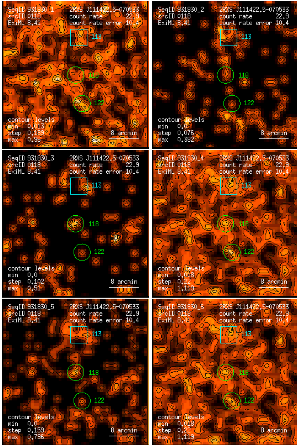
Figure 118: RASS 931830: detection 0118: band rate images, Gaussian filter: (1) PSPC channels 11 – 41, (2) 52 – 90, (3) 91 – 201, (4) 11 – 235, (5) 52 – 201, (6) 11 – 201. Broad band rates in counts/ks. Band rate contour levels in counts/ks/arcmin 2 .
