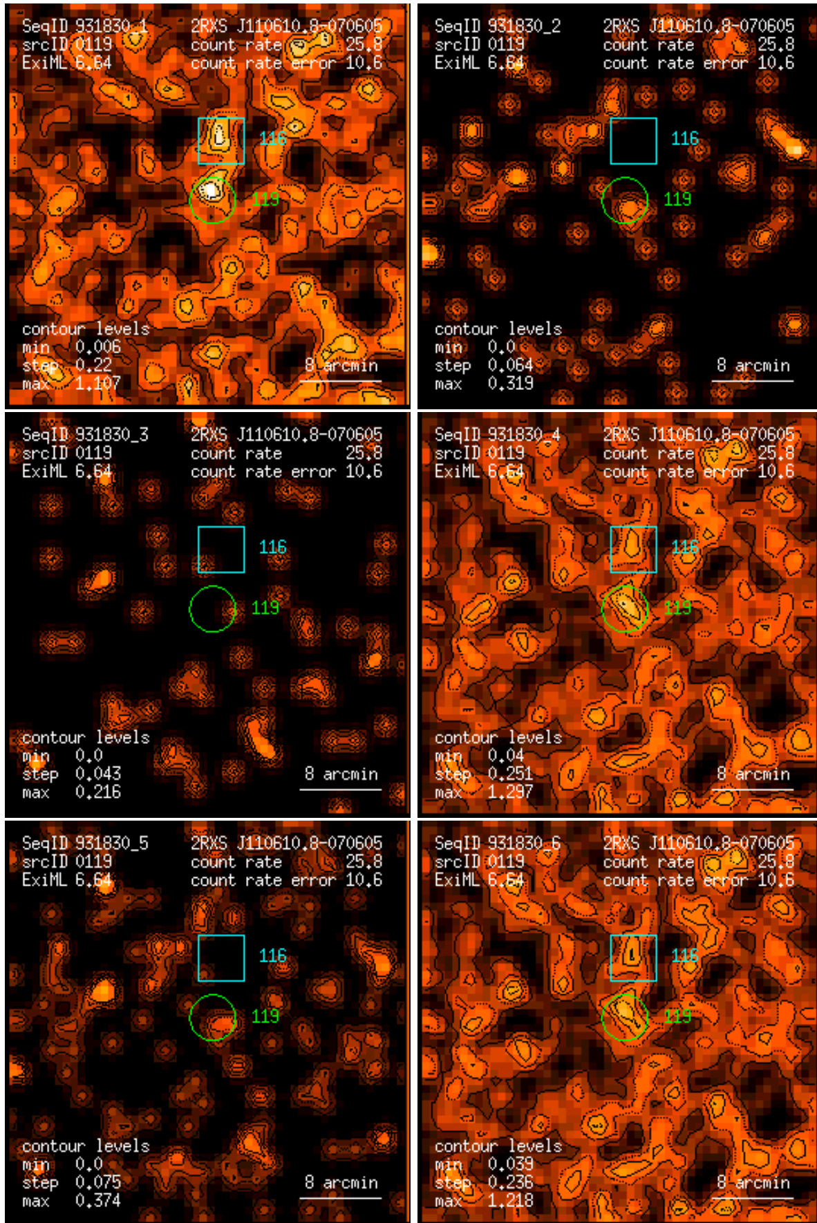
Figure 119: RASS 931830: detection 0119: band rate images, Gaussian filter: (1) PSPC channels 11 – 41, (2) 52 – 90, (3) 91 – 201, (4) 11 – 235, (5) 52 – 201, (6) 11 – 201. Broad band rates in counts/ks. Band rate contour levels in counts/ks/arcmin 2 .
