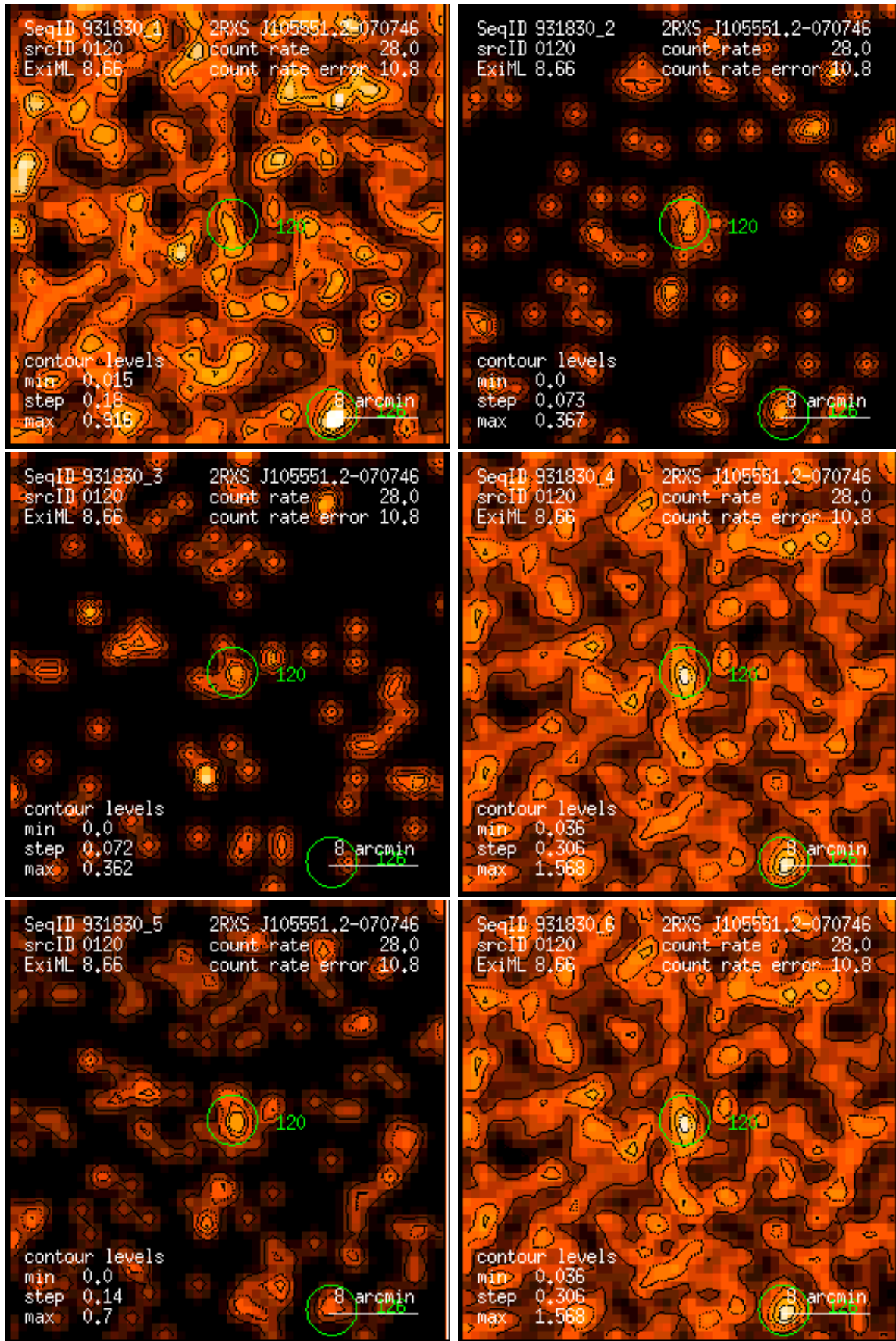
Figure 120: RASS 931830: detection 0120: band rate images, Gaussian filter: (1) PSPC channels 11 – 41, (2) 52 – 90, (3) 91 – 201, (4) 11 – 235, (5) 52 – 201, (6) 11 – 201. Broad band rates in counts/ks. Band rate contour levels in counts/ks/arcmin 2 .
