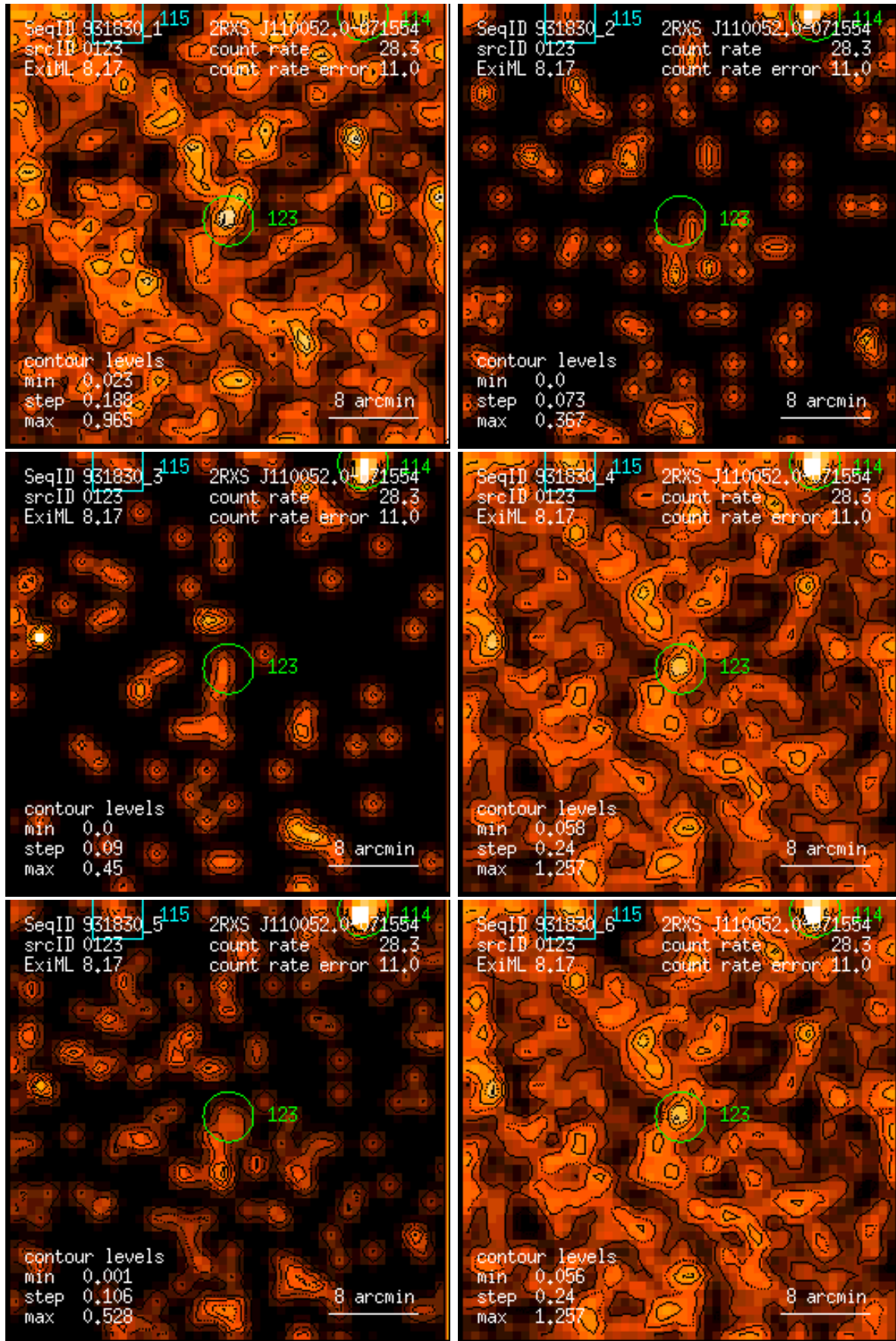
Figure 123: RASS 931830: detection 0123: band rate images, Gaussian filter: (1) PSPC channels 11 – 41, (2) 52 – 90, (3) 91 – 201, (4) 11 – 235, (5) 52 – 201, (6) 11 – 201. Broad band rates in counts/ks. Band rate contour levels in counts/ks/arcmin 2 .
