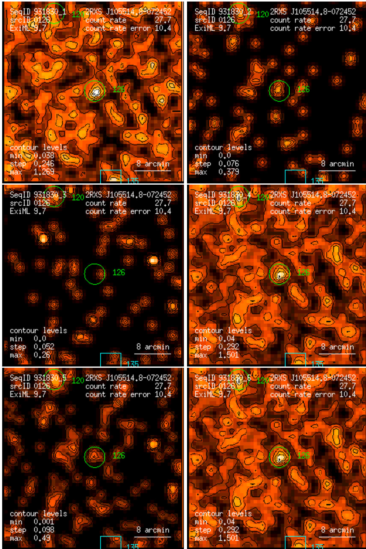
Figure 126: RASS 931830: detection 0126: band rate images, Gaussian filter: (1) PSPC channels 11 – 41, (2) 52 – 90, (3) 91 – 201, (4) 11 – 235, (5) 52 – 201, (6) 11 – 201. Broad band rates in counts/ks. Band rate contour levels in counts/ks/arcmin 2 .
