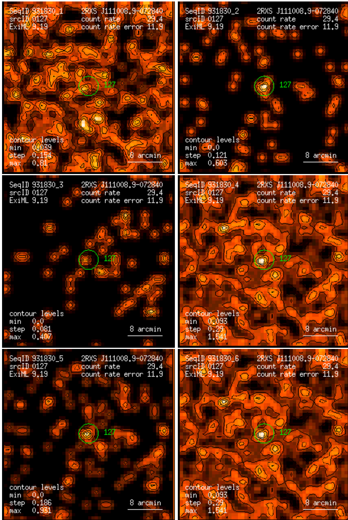
Figure 127: RASS 931830: detection 0127: band rate images, Gaussian filter: (1) PSPC channels 11 – 41, (2) 52 – 90, (3) 91 – 201, (4) 11 – 235, (5) 52 – 201, (6) 11 – 201. Broad band rates in counts/ks. Band rate contour levels in counts/ks/arcmin 2 .
