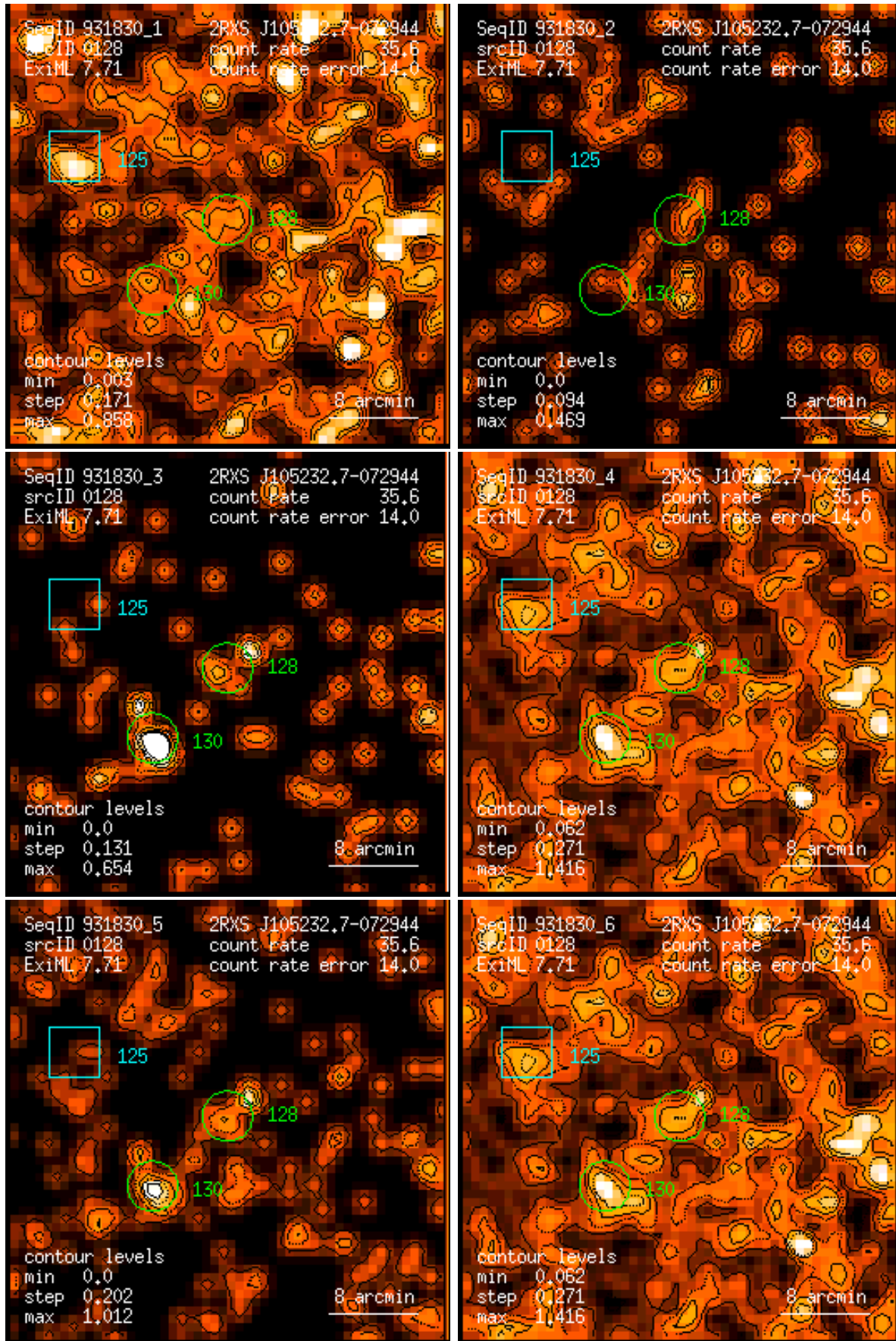
Figure 128: RASS 931830: detection 0128: band rate images, Gaussian filter: (1) PSPC channels 11 – 41, (2) 52 – 90, (3) 91 – 201, (4) 11 – 235, (5) 52 – 201, (6) 11 – 201. Broad band rates in counts/ks. Band rate contour levels in counts/ks/arcmin 2 .
