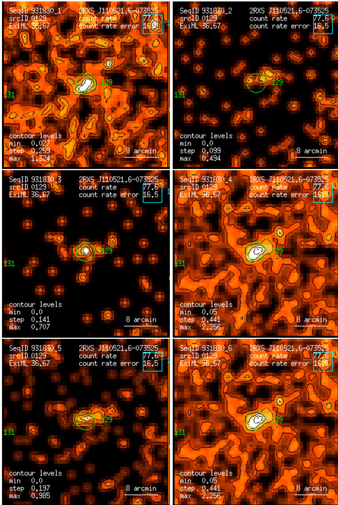
Figure 129: RASS 931830: detection 0129: band rate images, Gaussian filter: (1) PSPC channels 11 – 41, (2) 52 – 90, (3) 91 – 201, (4) 11 – 235, (5) 52 – 201, (6) 11 – 201. Broad band rates in counts/ks. Band rate contour levels in counts/ks/arcmin 2 .
