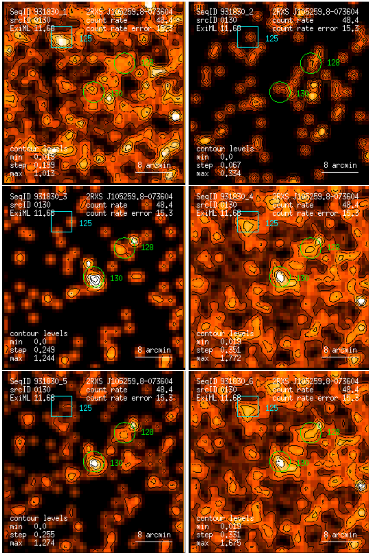
Figure 130: RASS 931830: detection 0130: band rate images, Gaussian filter: (1) PSPC channels 11 – 41, (2) 52 – 90, (3) 91 – 201, (4) 11 – 235, (5) 52 – 201, (6) 11 – 201. Broad band rates in counts/ks. Band rate contour levels in counts/ks/arcmin 2 .
