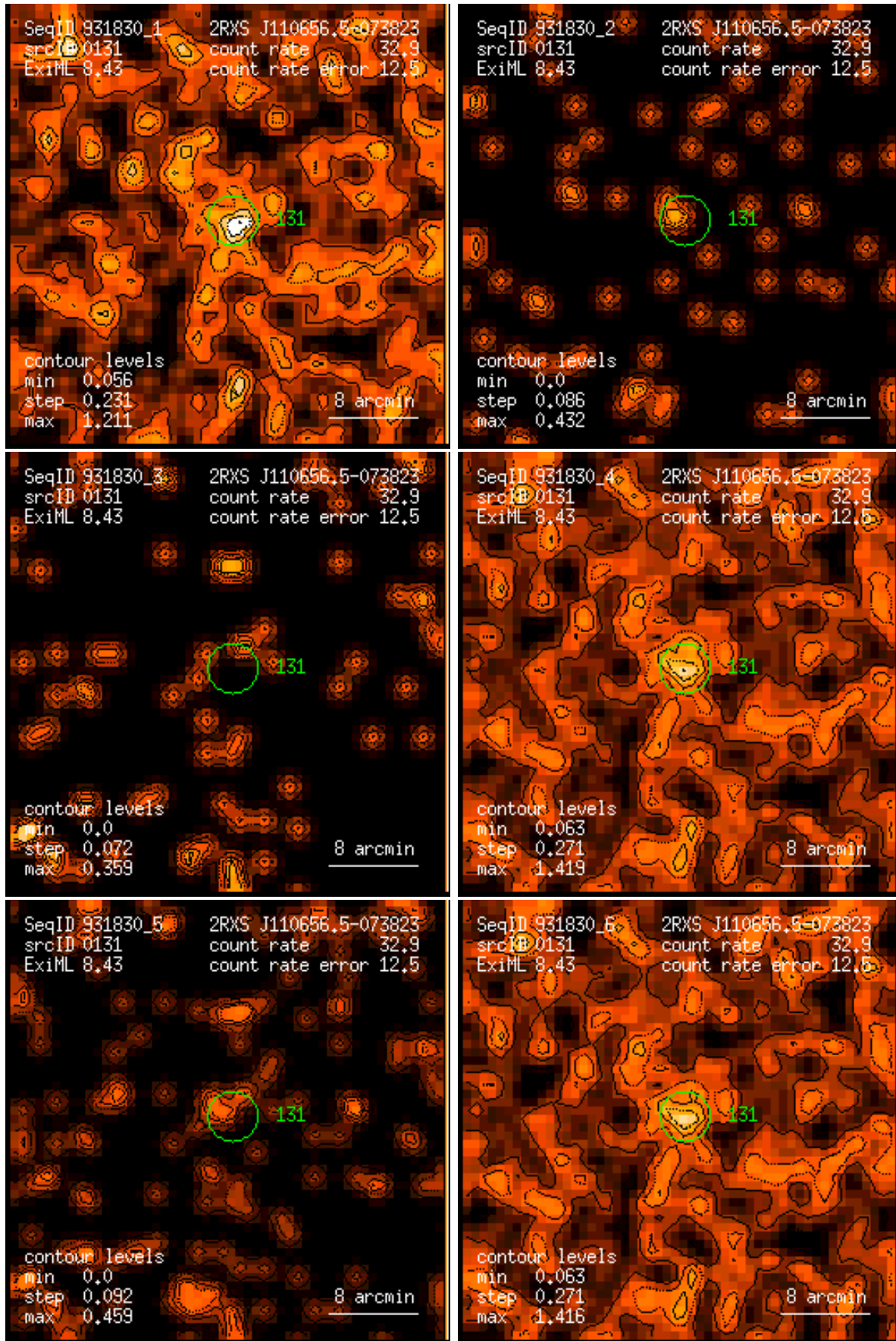
Figure 131: RASS 931830: detection 0131: band rate images, Gaussian filter: (1) PSPC channels 11 – 41, (2) 52 – 90, (3) 91 – 201, (4) 11 – 235, (5) 52 – 201, (6) 11 – 201. Broad band rates in counts/ks. Band rate contour levels in counts/ks/arcmin 2 .
