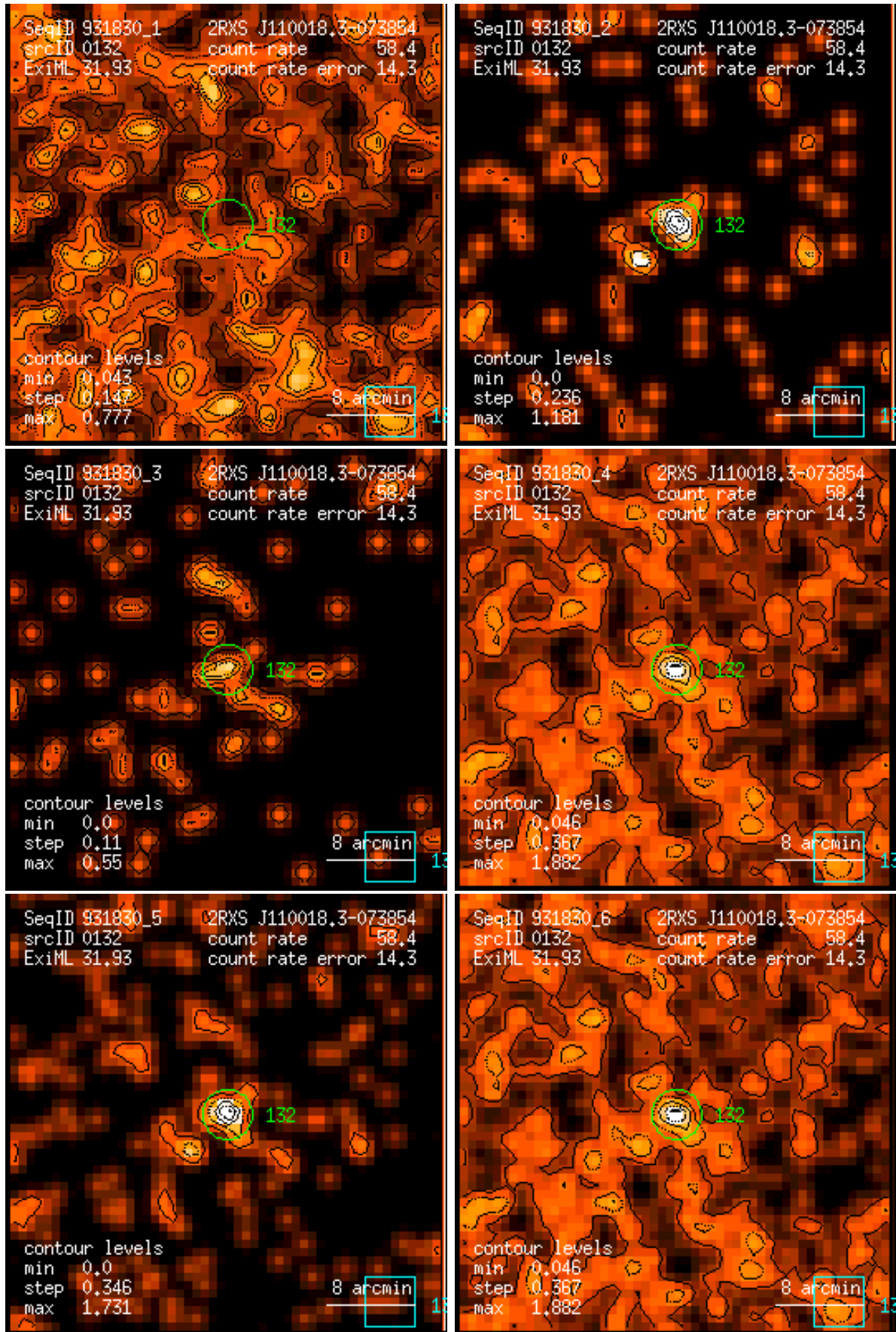
Figure 132: RASS 931830: detection 0132: band rate images, Gaussian filter: (1) PSPC channels 11 – 41, (2) 52 – 90, (3) 91 – 201, (4) 11 – 235, (5) 52 – 201, (6) 11 – 201. Broad band rates in counts/ks. Band rate contour levels in counts/ks/arcmin 2 .
