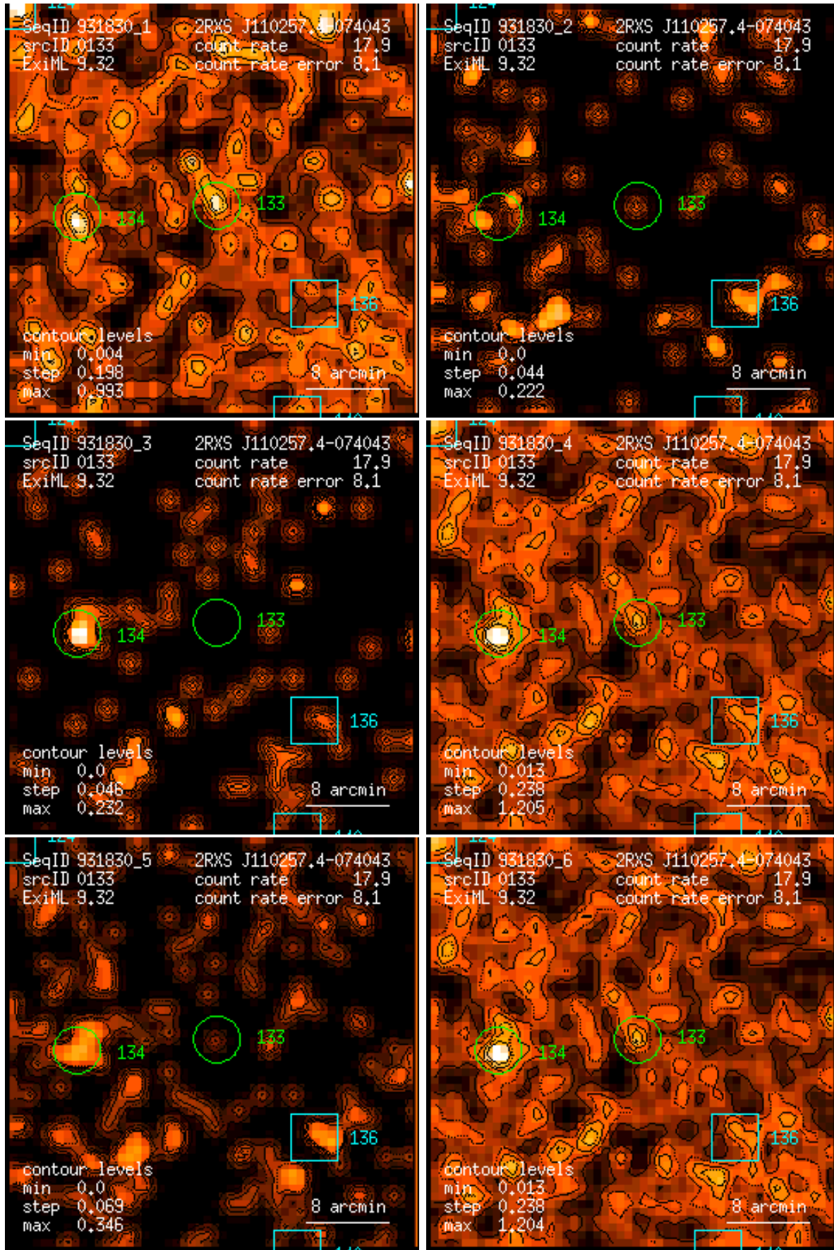
Figure 133: RASS 931830: detection 0133: band rate images, Gaussian filter: (1) PSPC channels 11 – 41, (2) 52 – 90, (3) 91 – 201, (4) 11 – 235, (5) 52 – 201, (6) 11 – 201. Broad band rates in counts/ks. Band rate contour levels in counts/ks/arcmin 2 .
