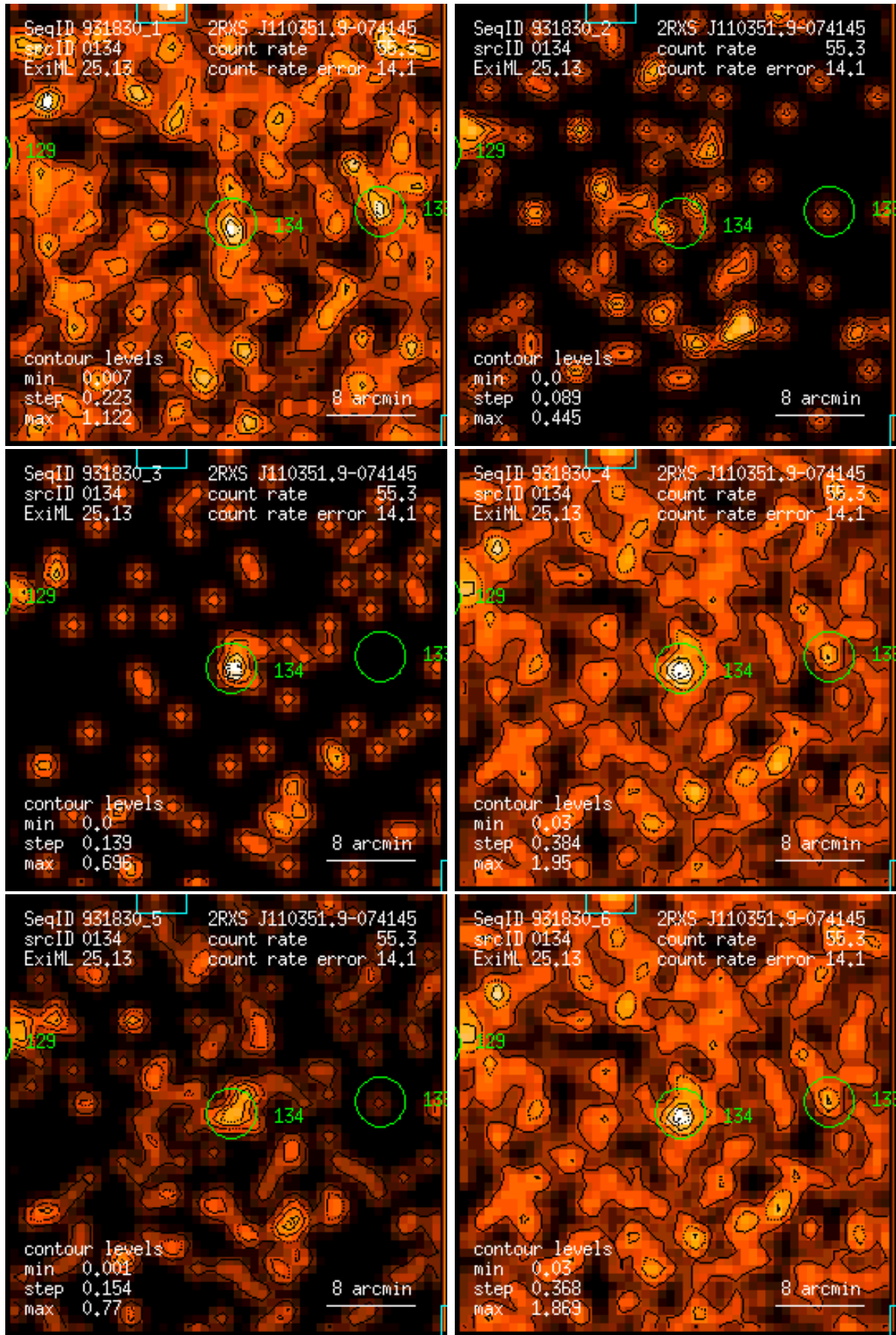
Figure 134: RASS 931830: detection 0134: band rate images, Gaussian filter: (1) PSPC channels 11 – 41, (2) 52 – 90, (3) 91 – 201, (4) 11 – 235, (5) 52 – 201, (6) 11 – 201. Broad band rates in counts/ks. Band rate contour levels in counts/ks/arcmin 2 .
