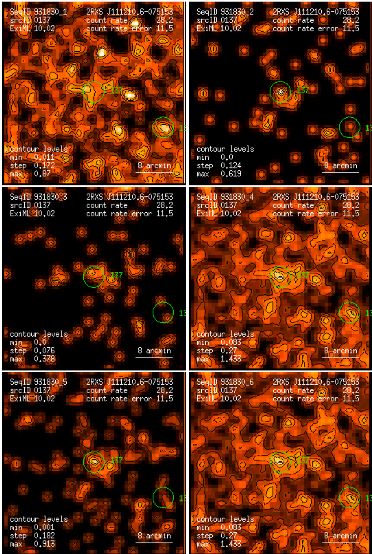
Figure 137: RASS 931830: detection 0137: band rate images, Gaussian filter: (1) PSPC channels 11 – 41, (2) 52 – 90, (3) 91 – 201, (4) 11 – 235, (5) 52 – 201, (6) 11 – 201. Broad band rates in counts/ks. Band rate contour levels in counts/ks/arcmin 2 .
