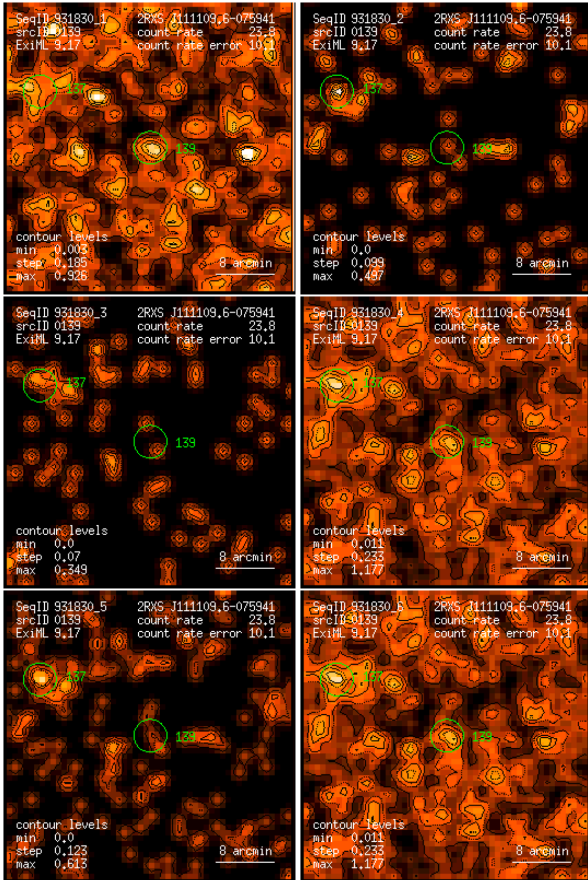
Figure 139: RASS 931830: detection 0139: band rate images, Gaussian filter: (1) PSPC channels 11 – 41, (2) 52 – 90, (3) 91 – 201, (4) 11 – 235, (5) 52 – 201, (6) 11 – 201. Broad band rates in counts/ks. Band rate contour levels in counts/ks/arcmin 2 .
