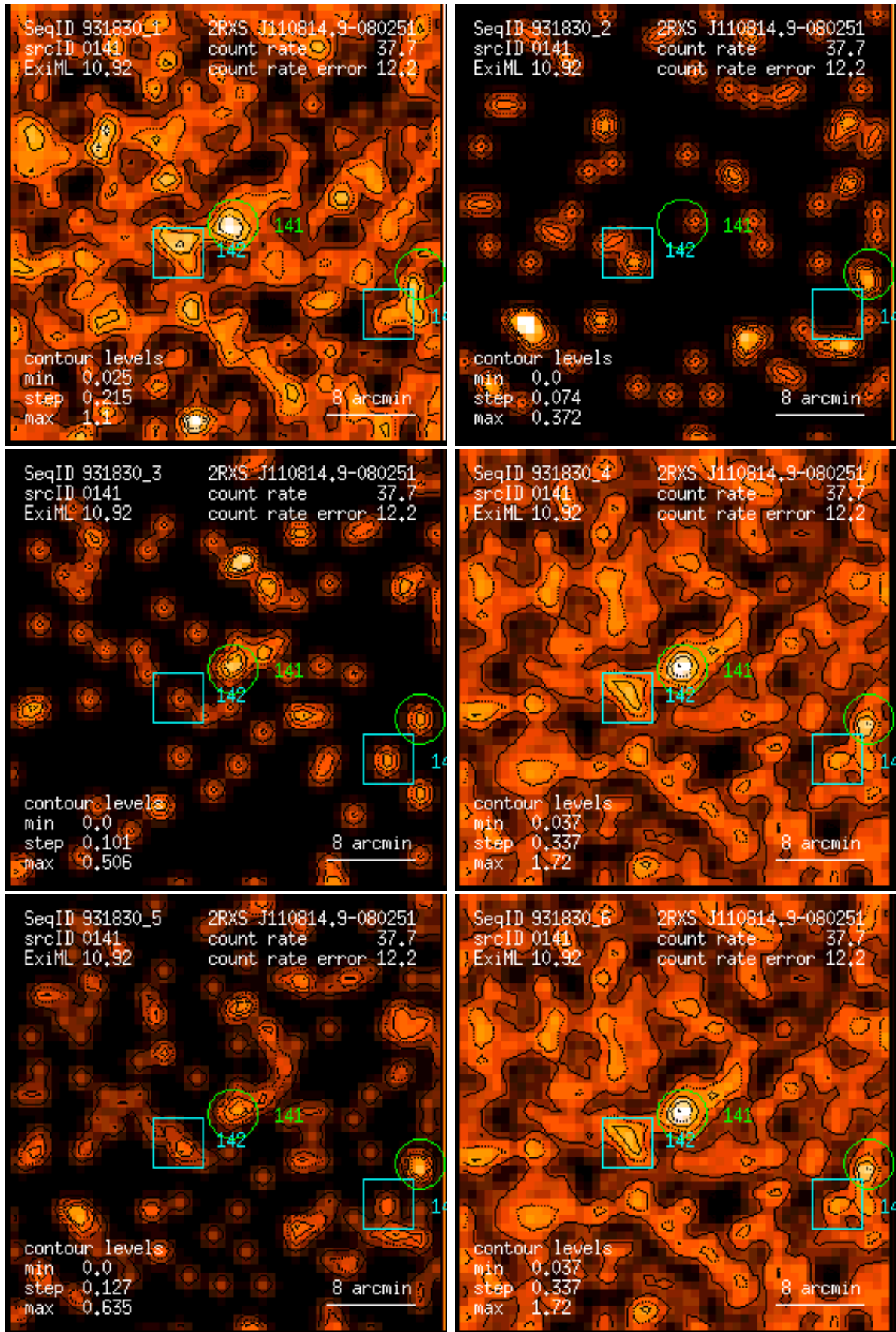
Figure 141: RASS 931830: detection 0141: band rate images, Gaussian filter: (1) PSPC channels 11 – 41, (2) 52 – 90, (3) 91 – 201, (4) 11 – 235, (5) 52 – 201, (6) 11 – 201. Broad band rates in counts/ks. Band rate contour levels in counts/ks/arcmin 2 .
