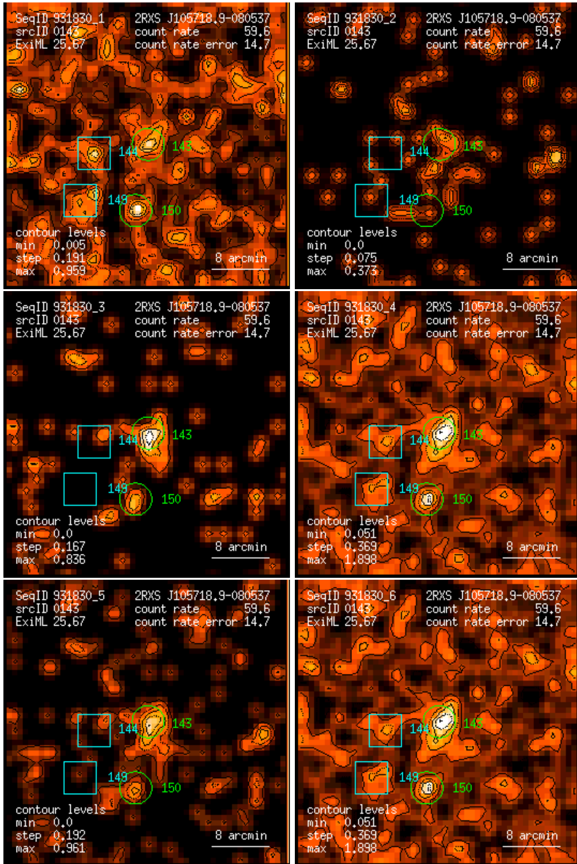
Figure 143: RASS 931830: detection 0143: band rate images, Gaussian filter: (1) PSPC channels 11 – 41, (2) 52 – 90, (3) 91 – 201, (4) 11 – 235, (5) 52 – 201, (6) 11 – 201. Broad band rates in counts/ks. Band rate contour levels in counts/ks/arcmin 2 .
