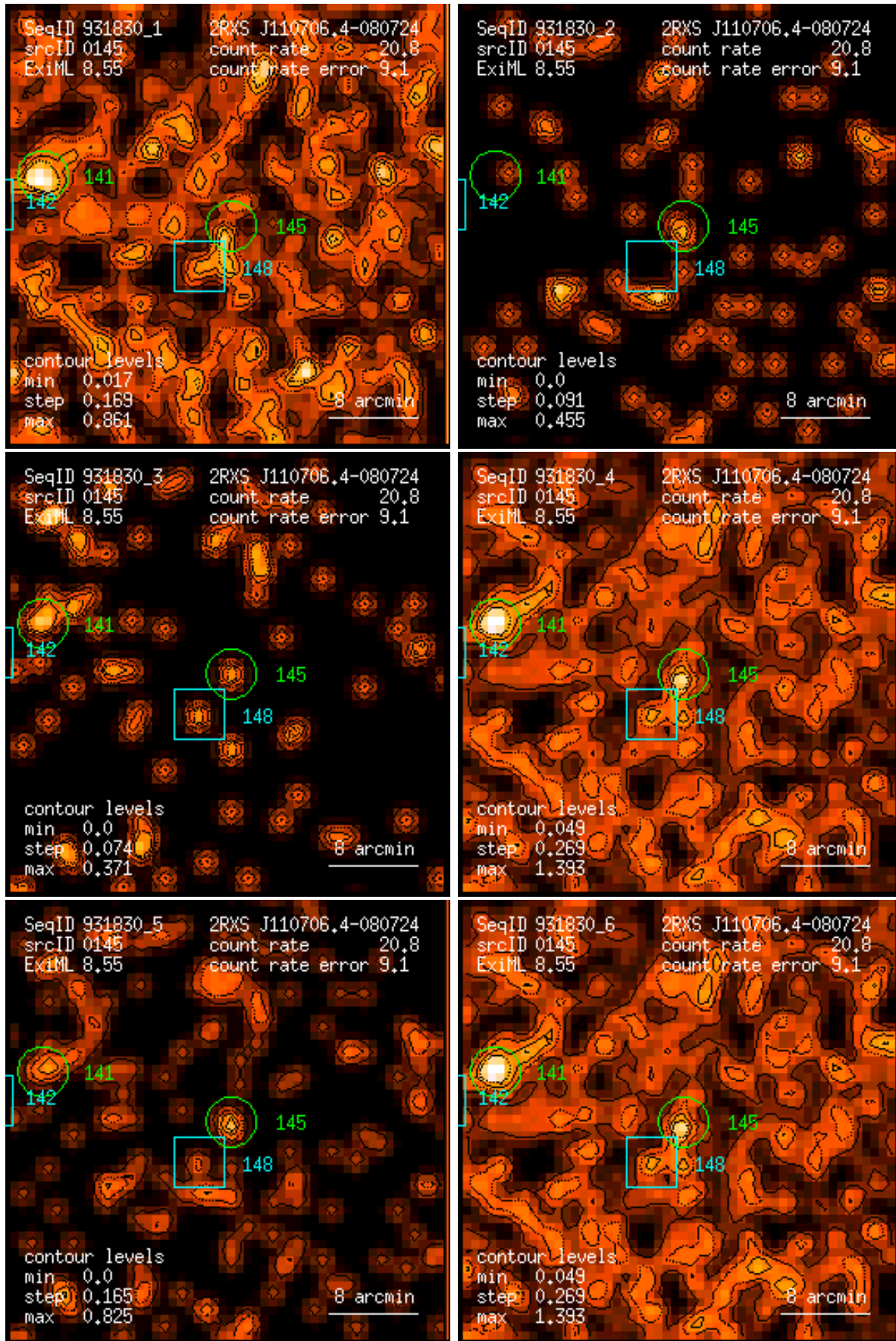
Figure 145: RASS 931830: detection 0145: band rate images, Gaussian filter: (1) PSPC channels 11 – 41, (2) 52 – 90, (3) 91 – 201, (4) 11 – 235, (5) 52 – 201, (6) 11 – 201. Broad band rates in counts/ks. Band rate contour levels in counts/ks/arcmin 2 .
