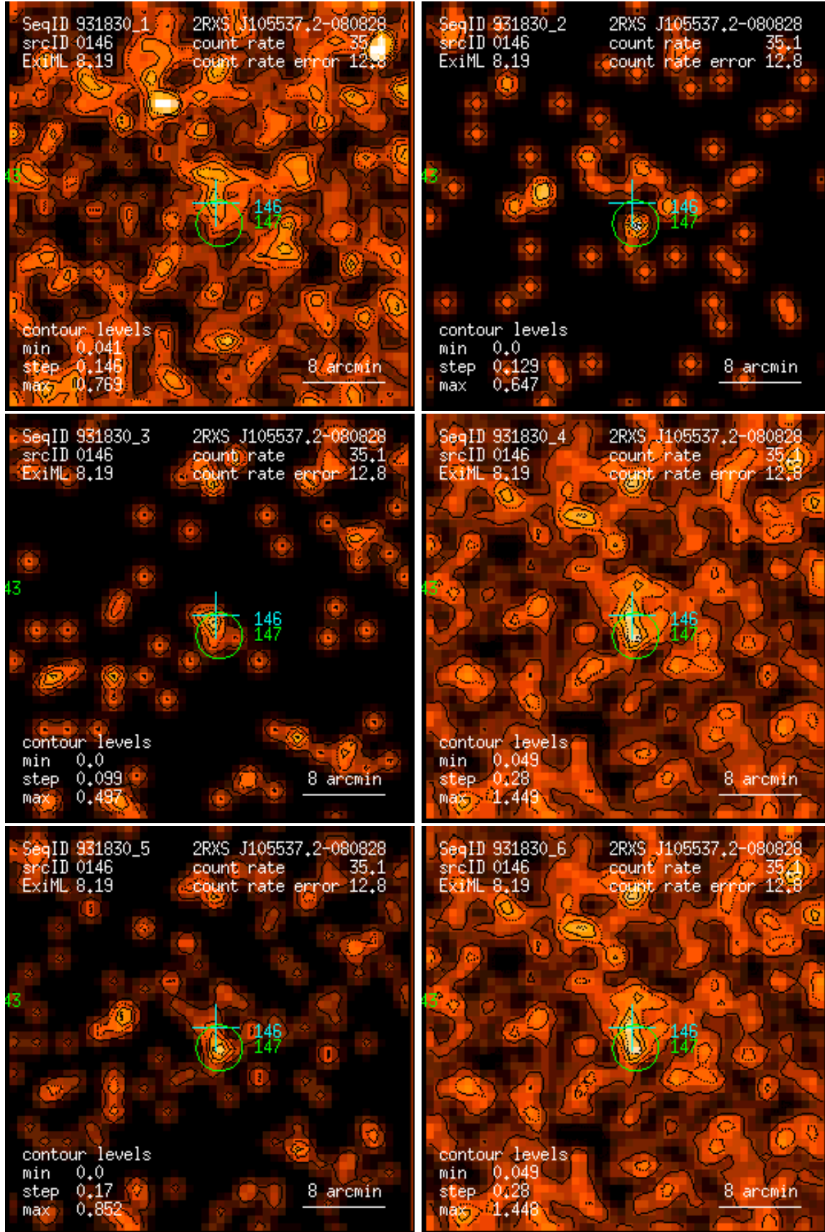
Figure 146: RASS 931830: detection 0146: band rate images, Gaussian filter: (1) PSPC channels 11 – 41, (2) 52 – 90, (3) 91 – 201, (4) 11 – 235, (5) 52 – 201, (6) 11 – 201. Broad band rates in counts/ks. Band rate contour levels in counts/ks/arcmin 2 .
