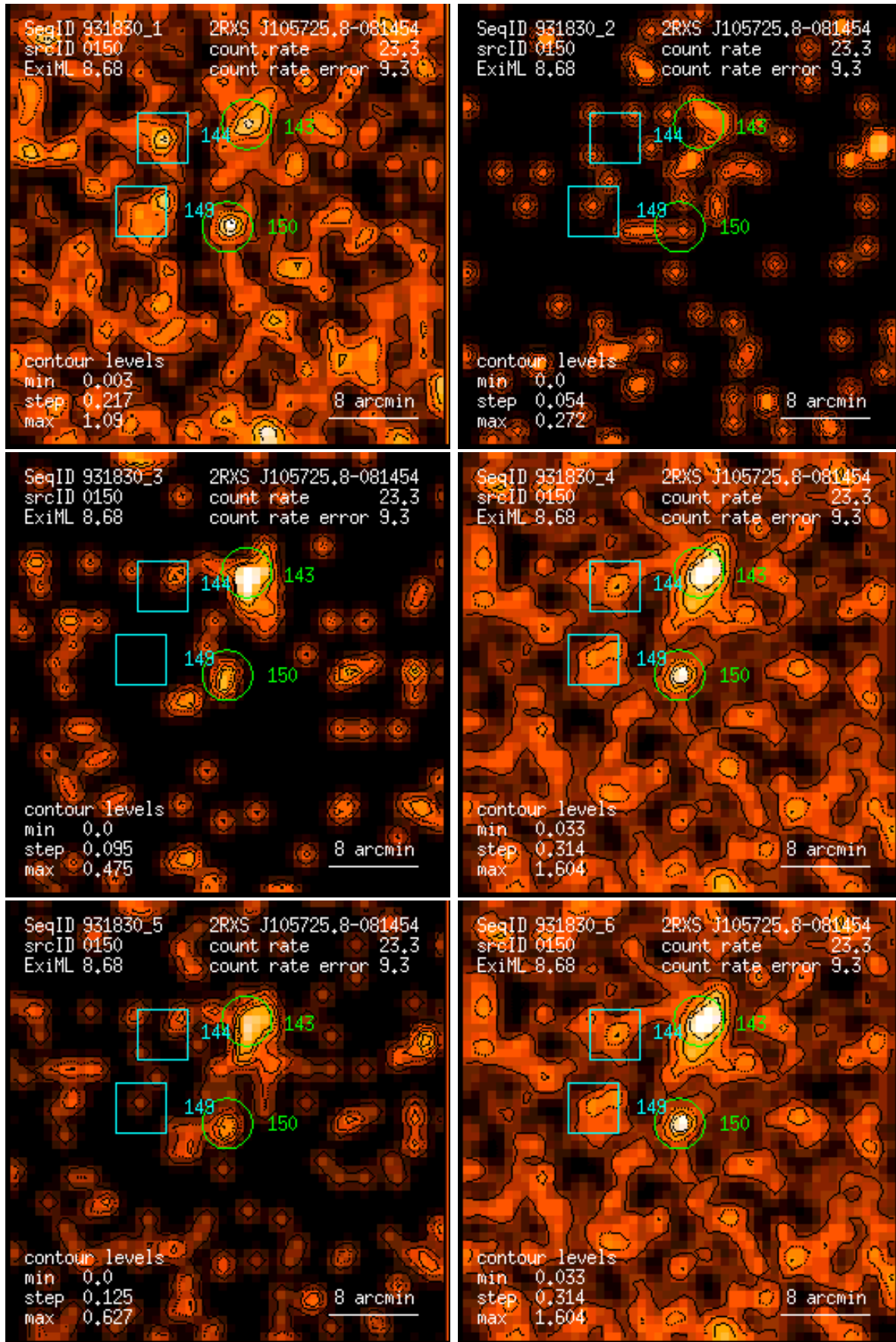
Figure 150: RASS 931830: detection 0150: band rate images, Gaussian filter: (1) PSPC channels 11 – 41, (2) 52 – 90, (3) 91 – 201, (4) 11 – 235, (5) 52 – 201, (6) 11 – 201. Broad band rates in counts/ks. Band rate contour levels in counts/ks/arcmin 2 .
