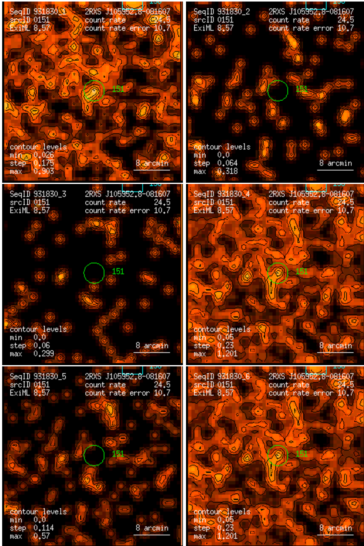
Figure 151: RASS 931830: detection 0151: band rate images, Gaussian filter: (1) PSPC channels 11 – 41, (2) 52 – 90, (3) 91 – 201, (4) 11 – 235, (5) 52 – 201, (6) 11 – 201. Broad band rates in counts/ks. Band rate contour levels in counts/ks/arcmin 2 .
