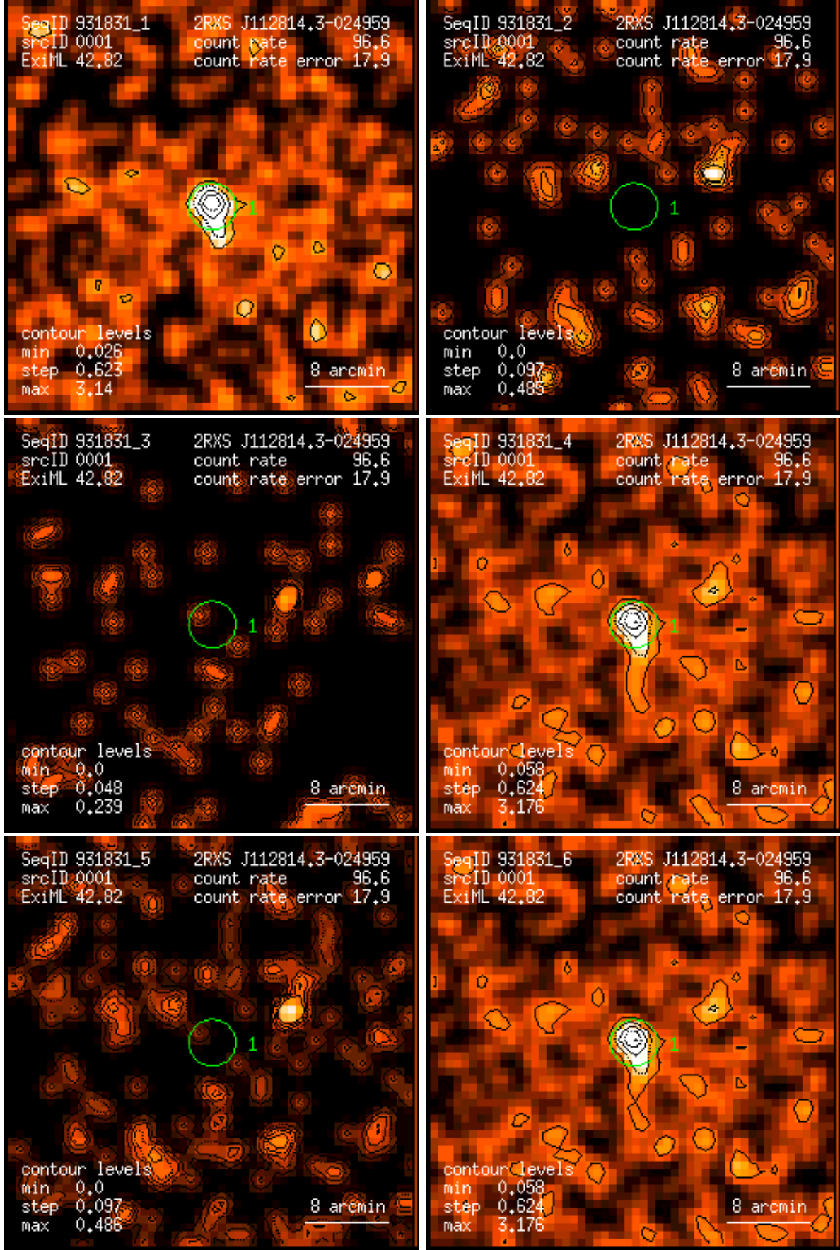
Figure 1: RASS 931831: detection 0001: band rate images, Gaussian filter: (1) PSPC channels 11 – 41, (2) 52 – 90, (3) 91 – 201, (4) 11 – 235, (5) 52 – 201, (6) 11 – 201. Broad band rates in counts/ks. Band rate contour levels in counts/ks/arcmin 2 .
