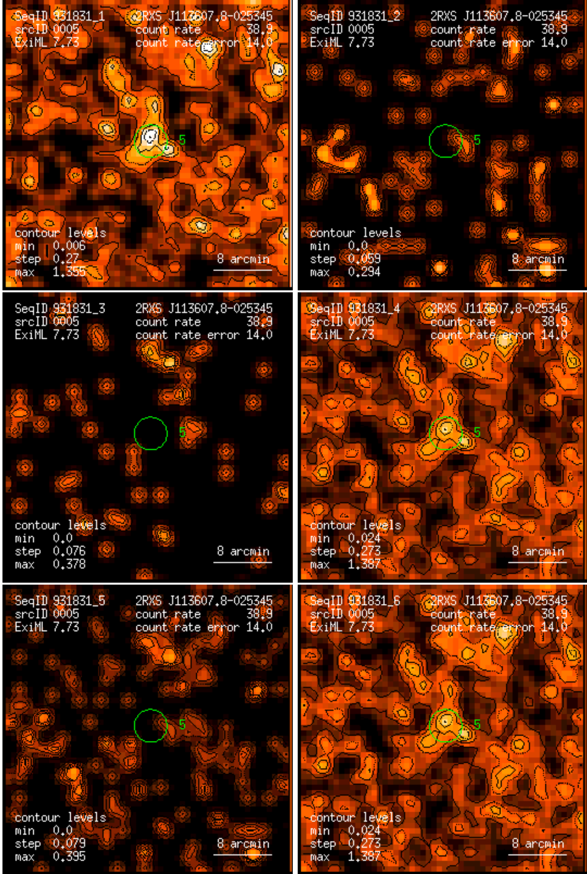
Figure 5: RASS 931831: detection 0005: band rate images, Gaussian filter: (1) PSPC channels 11 – 41, (2) 52 – 90, (3) 91 – 201, (4) 11 – 235, (5) 52 – 201, (6) 11 – 201. Broad band rates in counts/ks. Band rate contour levels in counts/ks/arcmin 2 .
