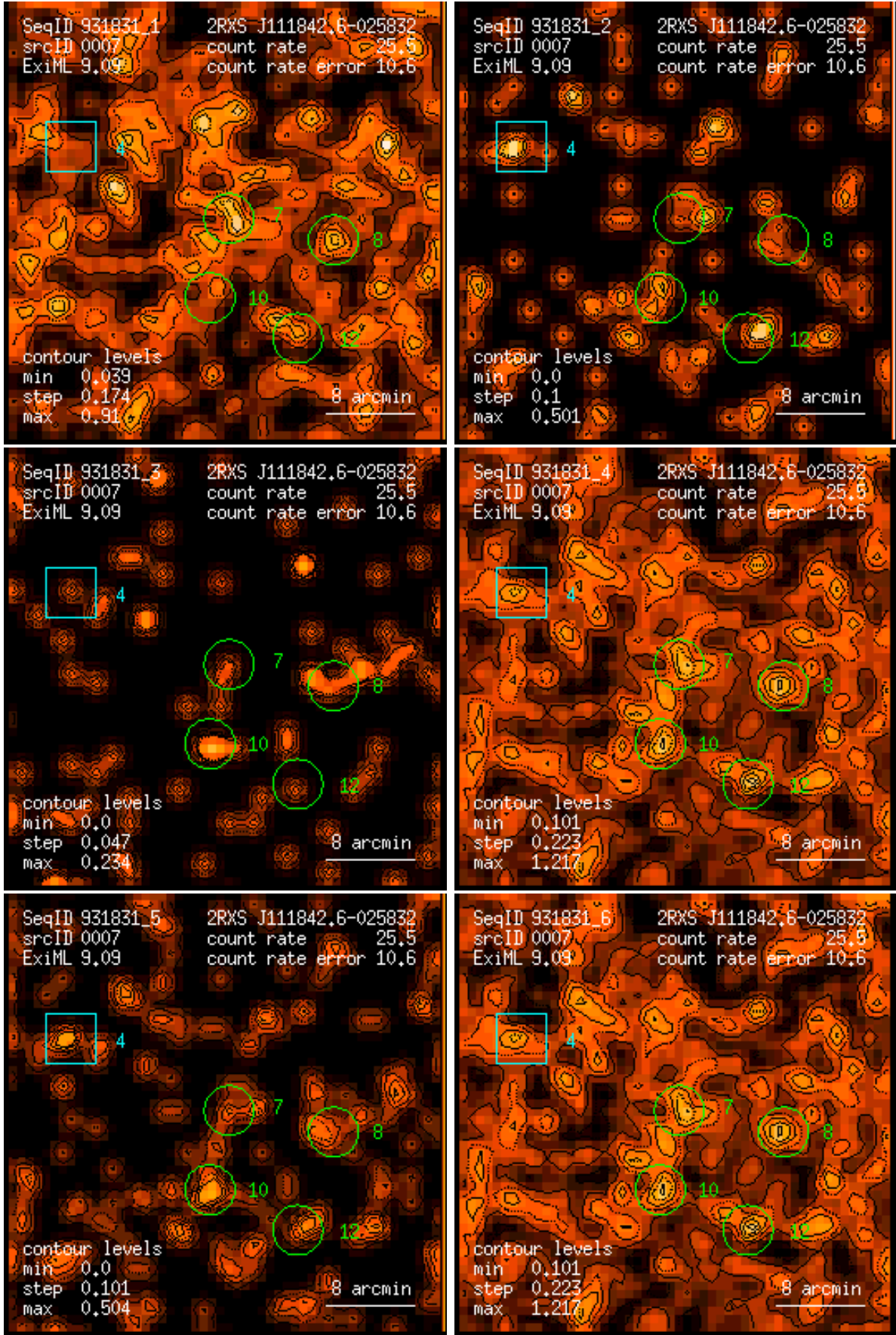
Figure 7: RASS 931831: detection 0007: band rate images, Gaussian filter: (1) PSPC channels 11 – 41, (2) 52 – 90, (3) 91 – 201, (4) 11 – 235, (5) 52 – 201, (6) 11 – 201. Broad band rates in counts/ks. Band rate contour levels in counts/ks/arcmin 2 .
