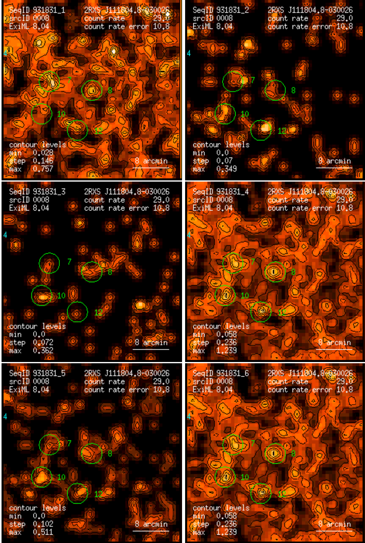
Figure 8: RASS 931831: detection 0008: band rate images, Gaussian filter: (1) PSPC channels 11 – 41, (2) 52 – 90, (3) 91 – 201, (4) 11 – 235, (5) 52 – 201, (6) 11 – 201. Broad band rates in counts/ks. Band rate contour levels in counts/ks/arcmin 2 .
