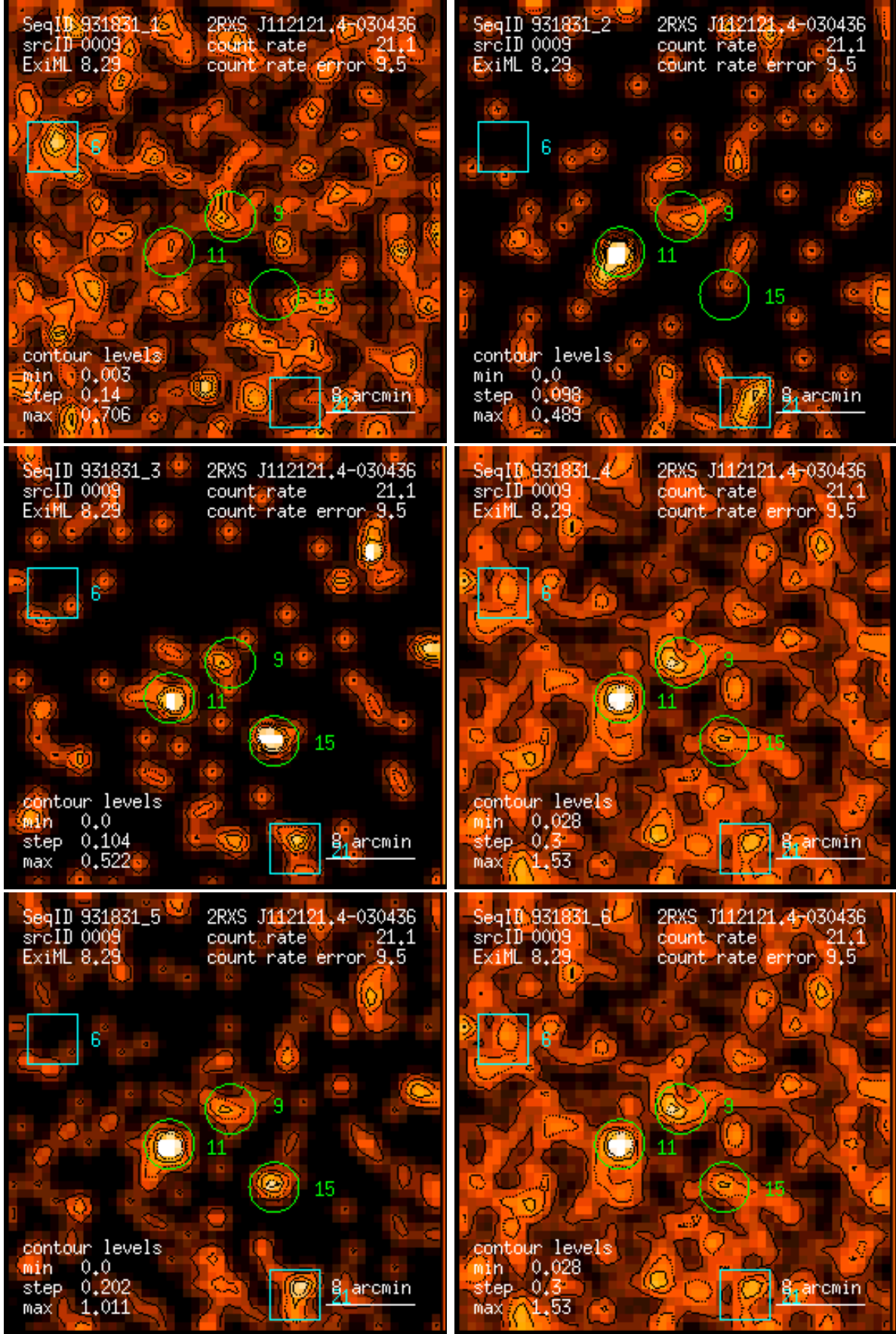
Figure 9: RASS 931831: detection 0009: band rate images, Gaussian filter: (1) PSPC channels 11 – 41, (2) 52 – 90, (3) 91 – 201, (4) 11 – 235, (5) 52 – 201, (6) 11 – 201. Broad band rates in counts/ks. Band rate contour levels in counts/ks/arcmin 2 .
