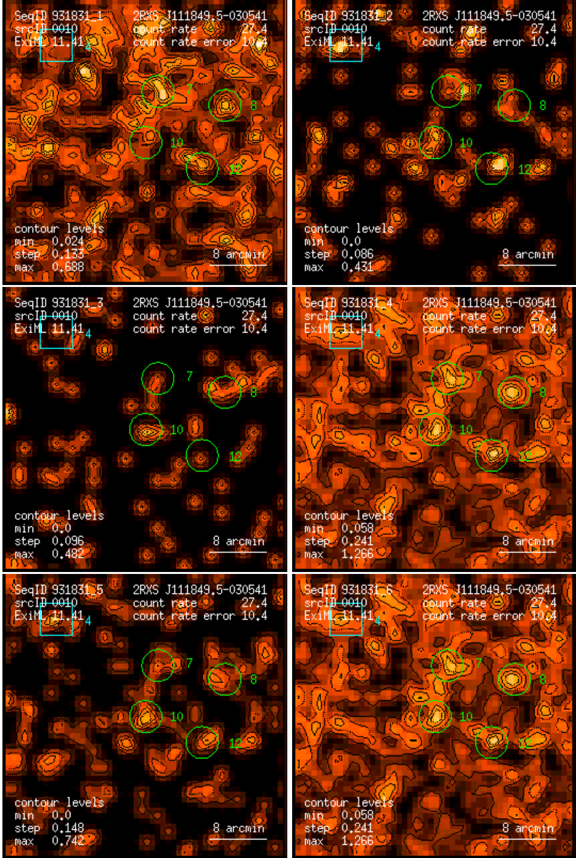
Figure 10: RASS 931831: detection 0010: band rate images, Gaussian filter: (1) PSPC channels 11 – 41, (2) 52 – 90, (3) 91 – 201, (4) 11 – 235, (5) 52 – 201, (6) 11 – 201. Broad band rates in counts/ks. Band rate contour levels in counts/ks/arcmin 2 .
