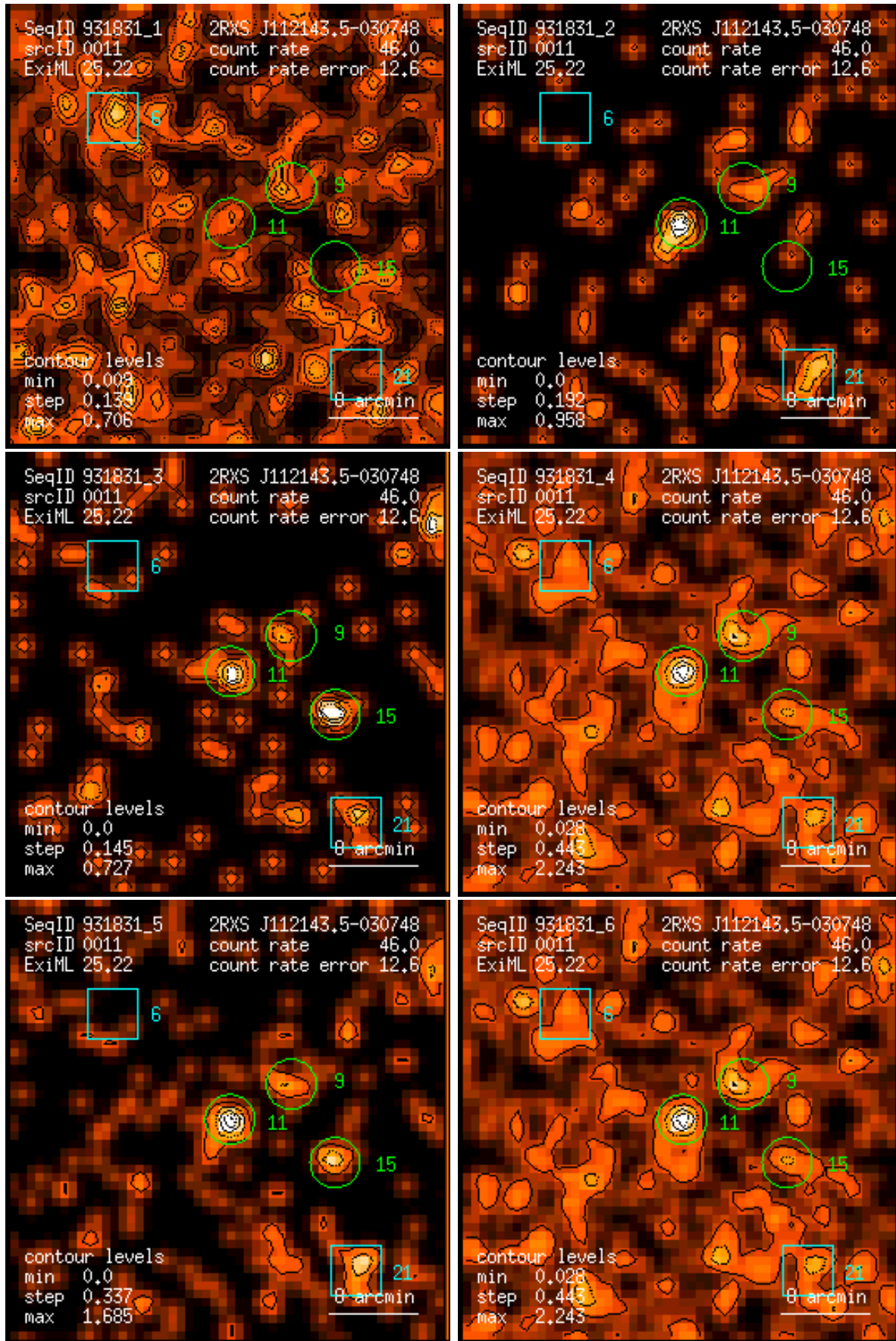
Figure 11: RASS 931831: detection 0011: band rate images, Gaussian filter: (1) PSPC channels 11 – 41, (2) 52 – 90, (3) 91 – 201, (4) 11 – 235, (5) 52 – 201, (6) 11 – 201. Broad band rates in counts/ks. Band rate contour levels in counts/ks/arcmin 2 .
