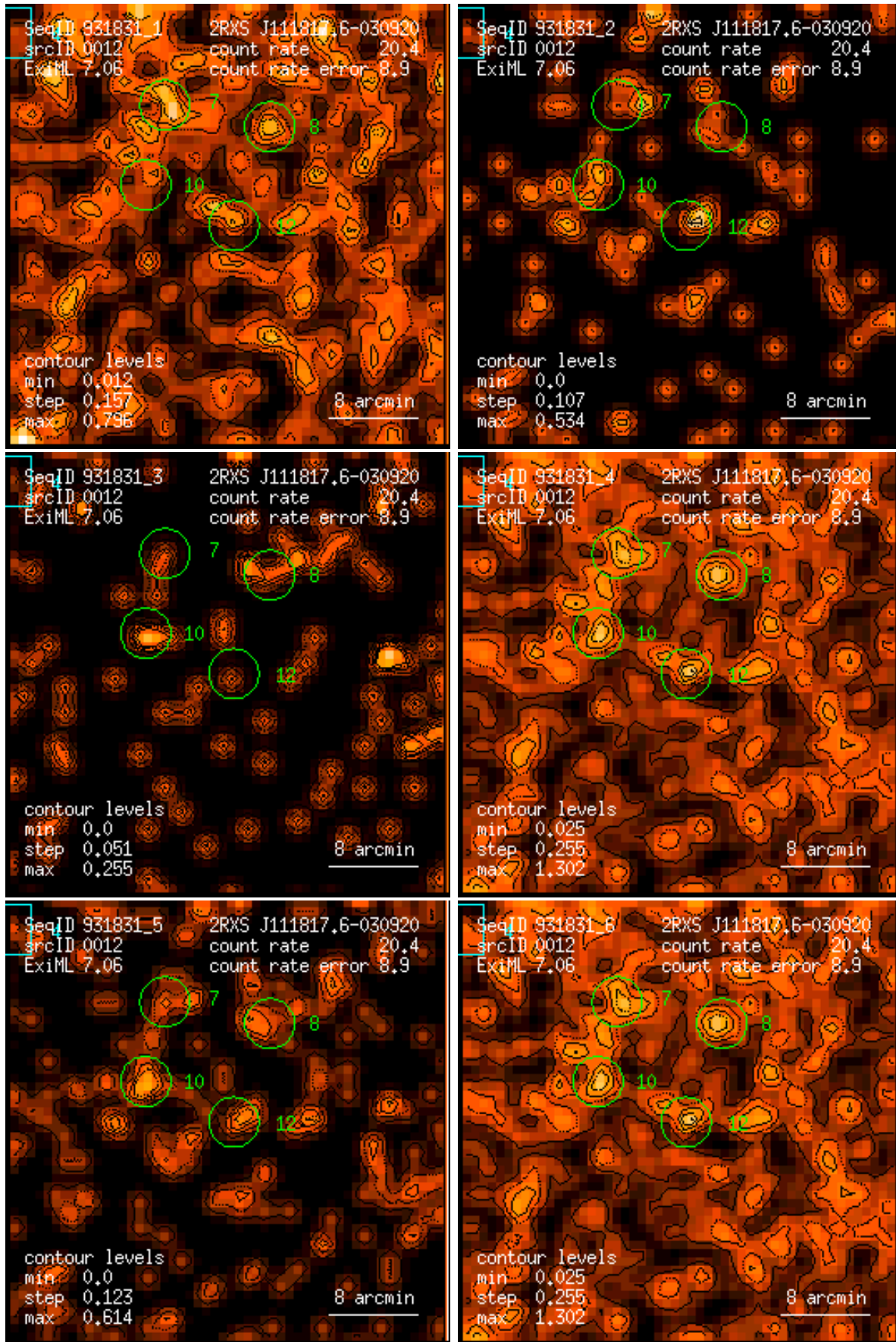
Figure 12: RASS 931831: detection 0012: band rate images, Gaussian filter: (1) PSPC channels 11 – 41, (2) 52 – 90, (3) 91 – 201, (4) 11 – 235, (5) 52 – 201, (6) 11 – 201. Broad band rates in counts/ks. Band rate contour levels in counts/ks/arcmin 2 .
