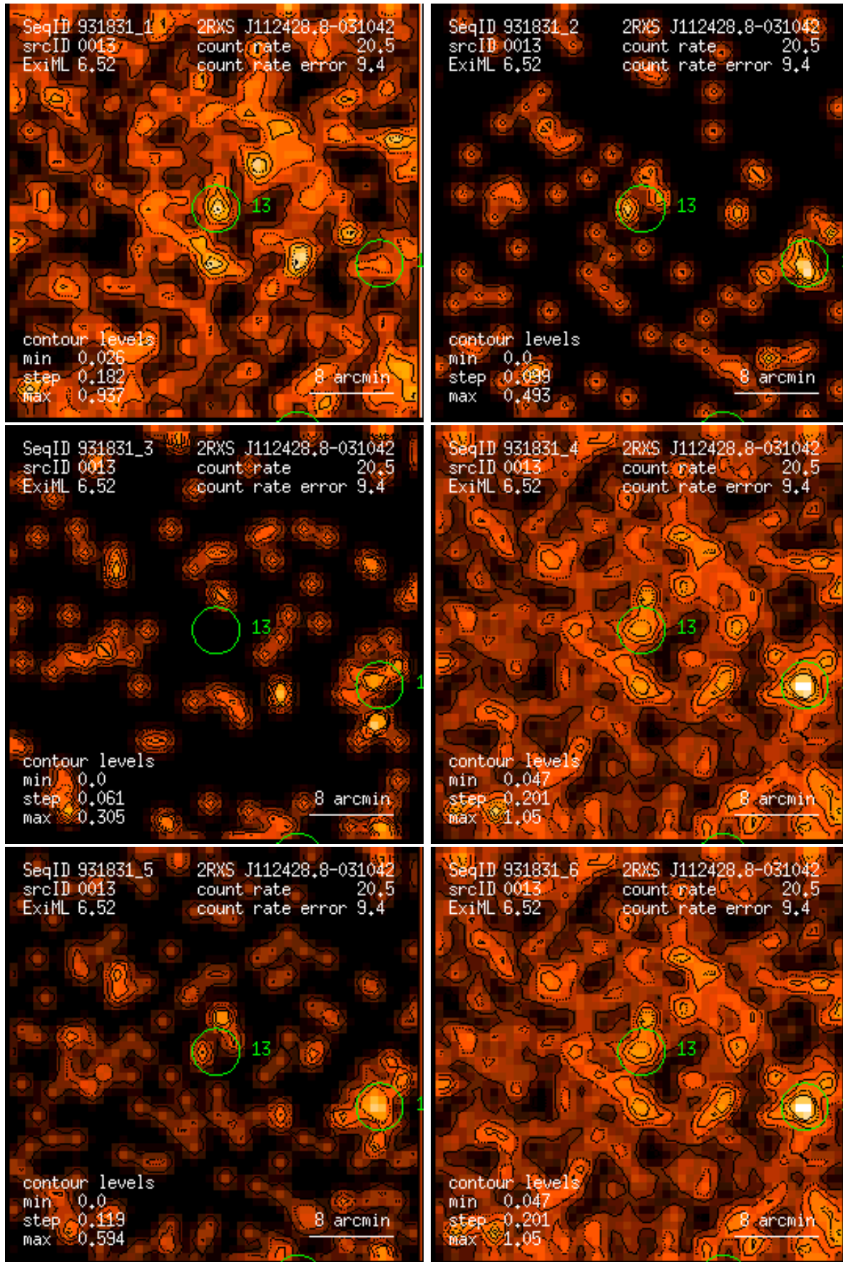
Figure 13: RASS 931831: detection 0013: band rate images, Gaussian filter: (1) PSPC channels 11 – 41, (2) 52 – 90, (3) 91 – 201, (4) 11 – 235, (5) 52 – 201, (6) 11 – 201. Broad band rates in counts/ks. Band rate contour levels in counts/ks/arcmin 2 .
