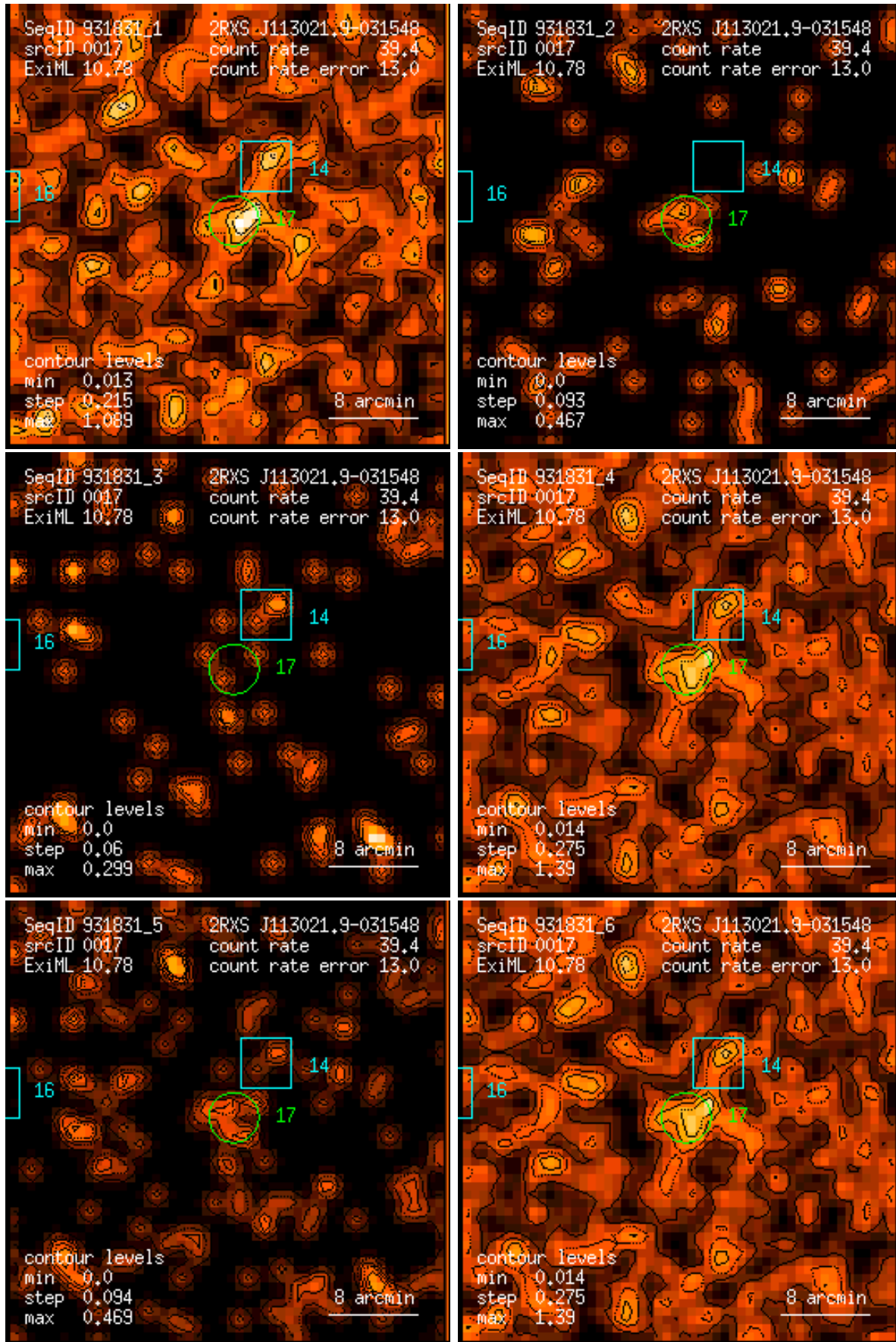
Figure 17: RASS 931831: detection 0017: band rate images, Gaussian filter: (1) PSPC channels 11 – 41, (2) 52 – 90, (3) 91 – 201, (4) 11 – 235, (5) 52 – 201, (6) 11 – 201. Broad band rates in counts/ks. Band rate contour levels in counts/ks/arcmin 2 .
