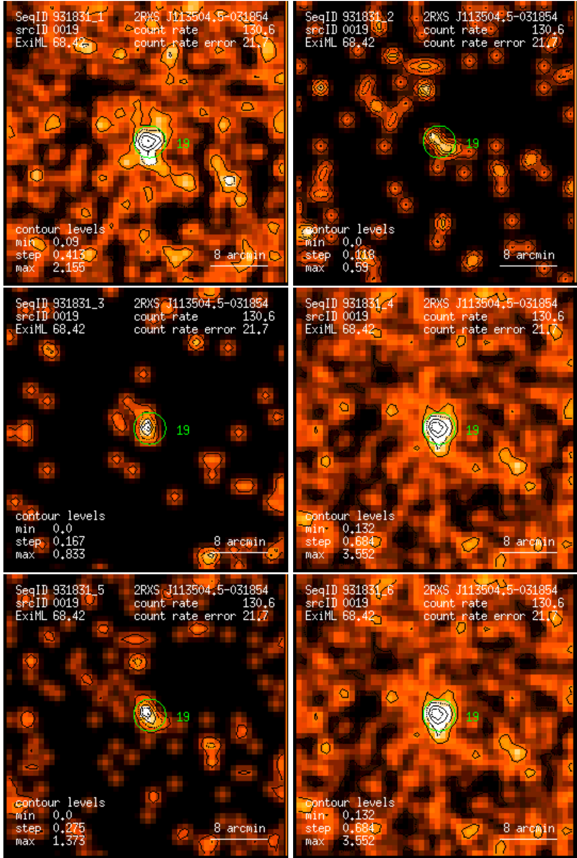
Figure 19: RASS 931831: detection 0019: band rate images, Gaussian filter: (1) PSPC channels 11 – 41, (2) 52 – 90, (3) 91 – 201, (4) 11 – 235, (5) 52 – 201, (6) 11 – 201. Broad band rates in counts/ks. Band rate contour levels in counts/ks/arcmin 2 .
