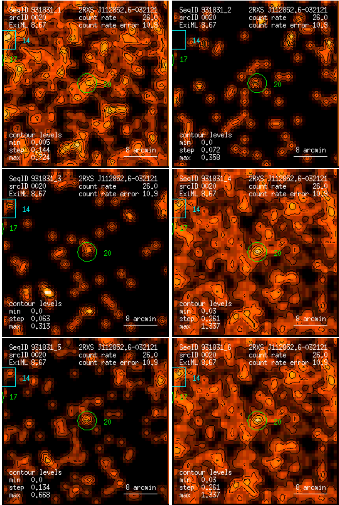
Figure 20: RASS 931831: detection 0020: band rate images, Gaussian filter: (1) PSPC channels 11 – 41, (2) 52 – 90, (3) 91 – 201, (4) 11 – 235, (5) 52 – 201, (6) 11 – 201. Broad band rates in counts/ks. Band rate contour levels in counts/ks/arcmin 2 .
