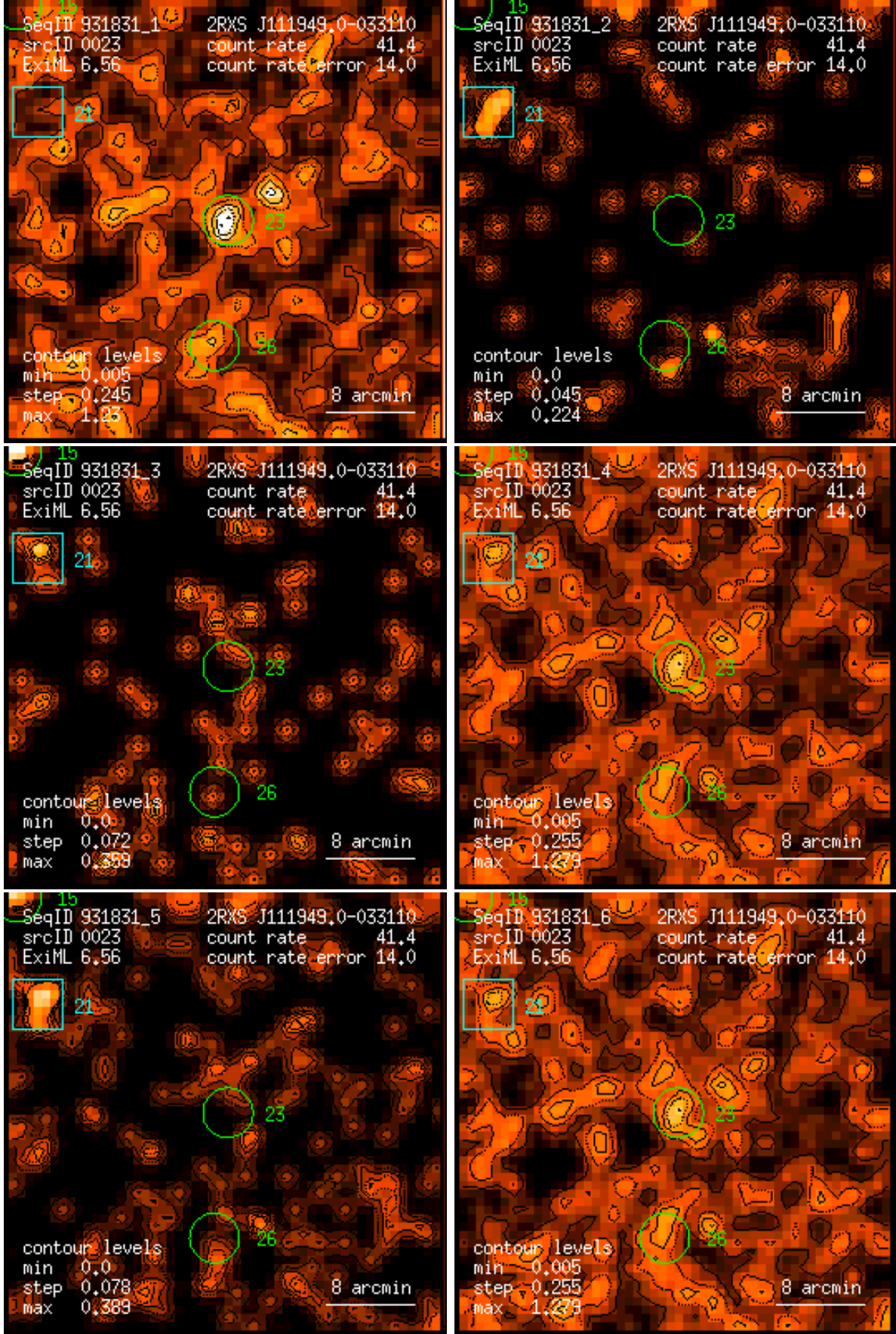
Figure 23: RASS 931831: detection 0023: band rate images, Gaussian filter: (1) PSPC channels 11 – 41, (2) 52 – 90, (3) 91 – 201, (4) 11 – 235, (5) 52 – 201, (6) 11 – 201. Broad band rates in counts/ks. Band rate contour levels in counts/ks/arcmin 2 .
